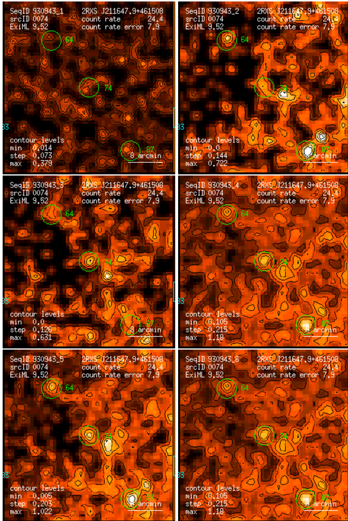
Figure 74: RASS 930943: detection 0074: band rate images, Gaussian filter: (1) PSPC channels 11 – 41, (2) 52 – 90, (3) 91 – 201, (4) 11 – 235, (5) 52 – 201, (6) 11 – 201. Broad band rates in counts/ks. Band rate contour levels in counts/ks/arcmin 2 .
