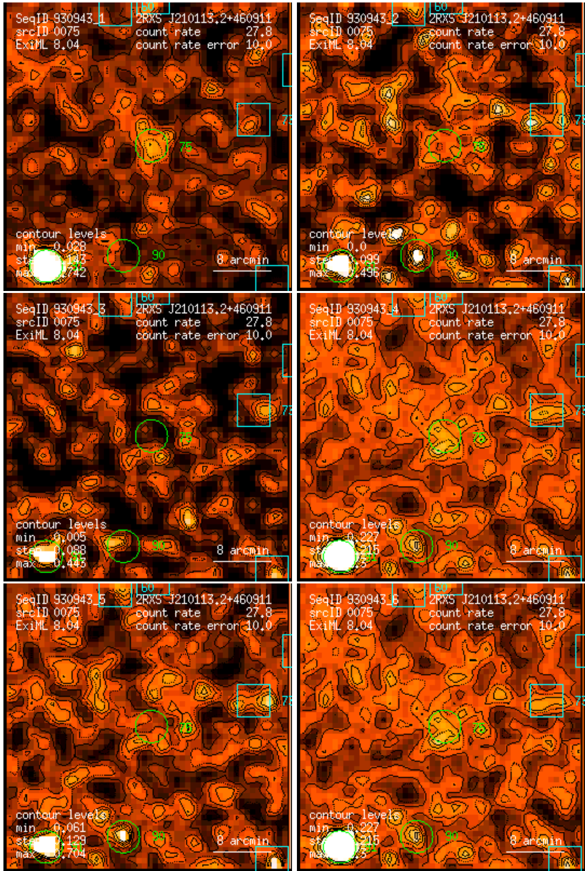
Figure 75: RASS 930943: detection 0075: band rate images, Gaussian filter: (1) PSPC channels 11 – 41, (2) 52 – 90, (3) 91 – 201, (4) 11 – 235, (5) 52 – 201, (6) 11 – 201. Broad band rates in counts/ks. Band rate contour levels in counts/ks/arcmin 2 .
