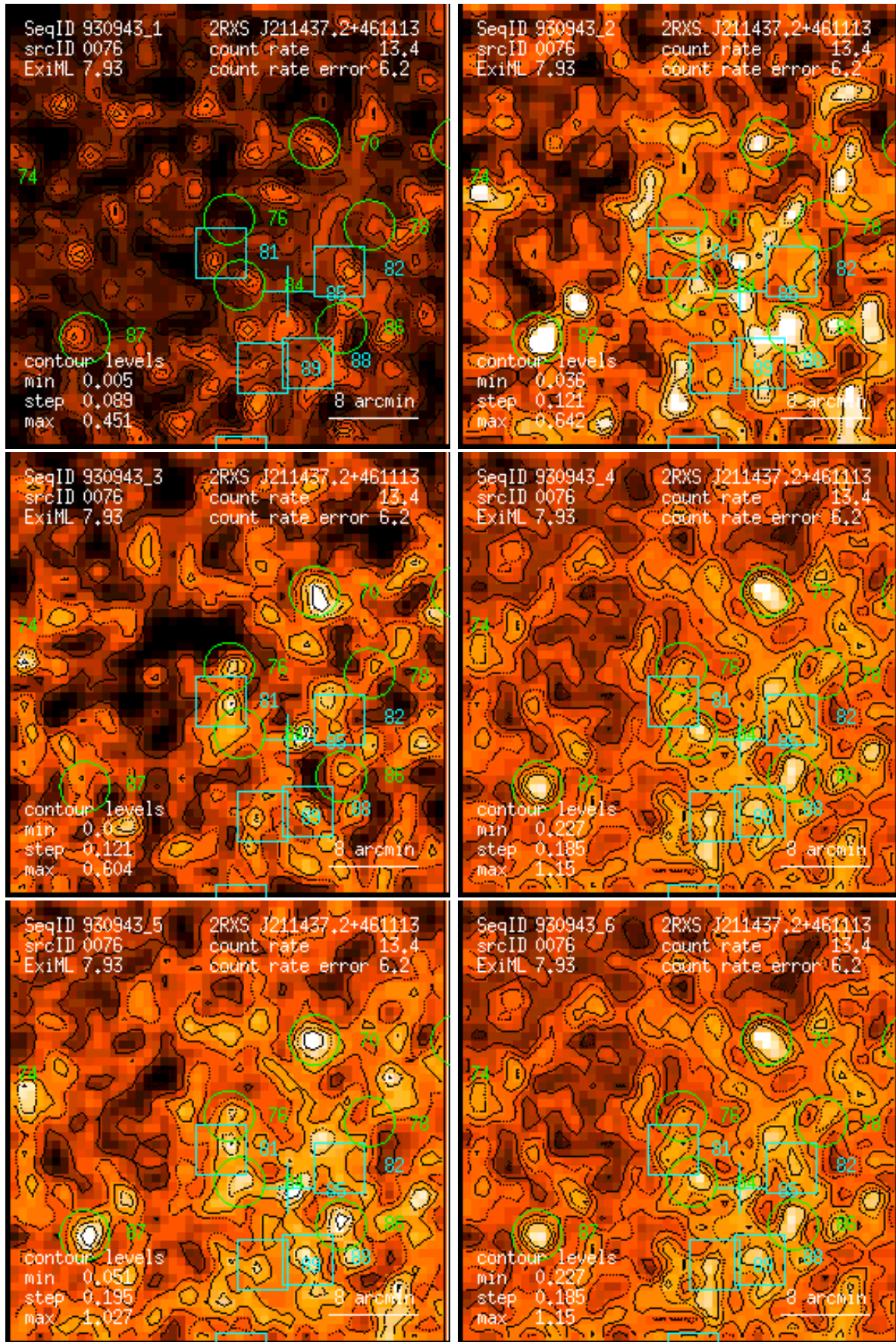
Figure 76: RASS 930943: detection 0076: band rate images, Gaussian filter: (1) PSPC channels 11 – 41, (2) 52 – 90, (3) 91 – 201, (4) 11 – 235, (5) 52 – 201, (6) 11 – 201. Broad band rates in counts/ks. Band rate contour levels in counts/ks/arcmin 2 .
