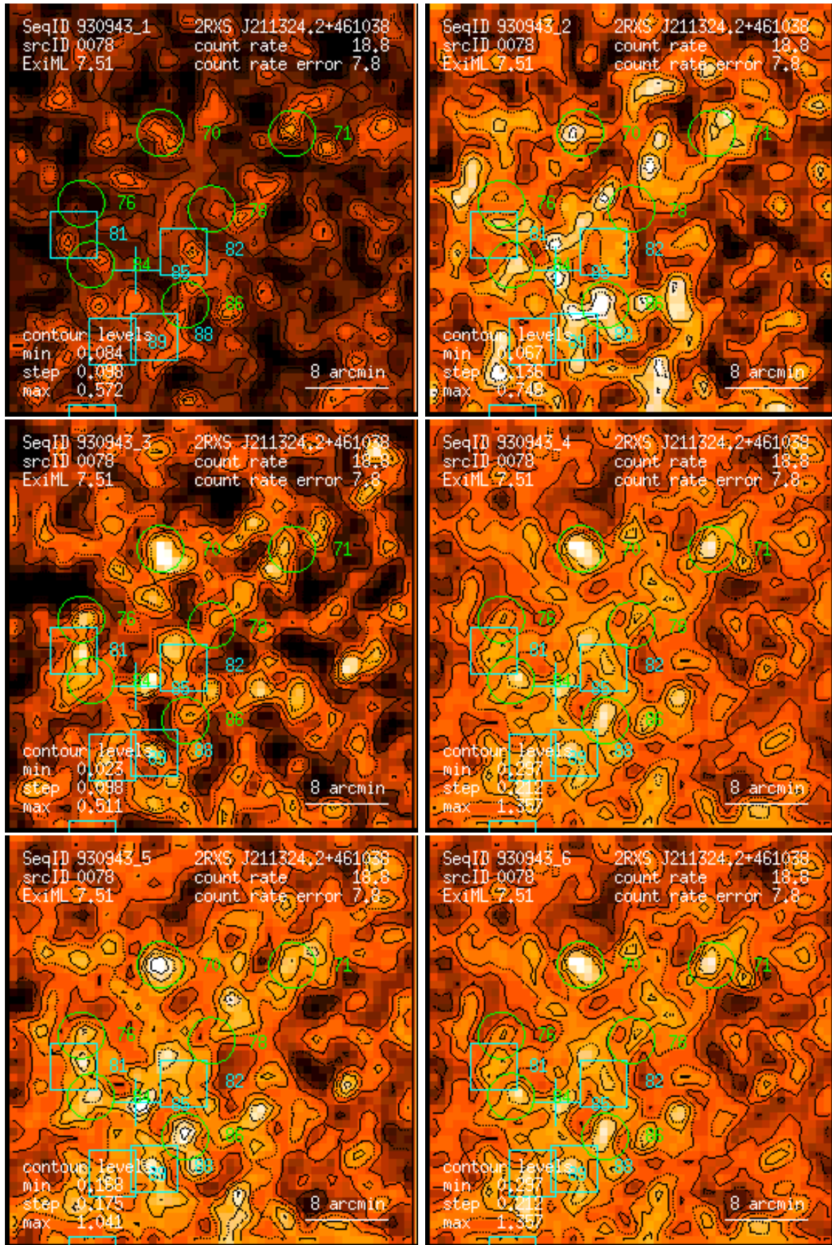
Figure 78: RASS 930943: detection 0078: band rate images, Gaussian filter: (1) PSPC channels 11 – 41, (2) 52 – 90, (3) 91 – 201, (4) 11 – 235, (5) 52 – 201, (6) 11 – 201. Broad band rates in counts/ks. Band rate contour levels in counts/ks/arcmin 2 .
