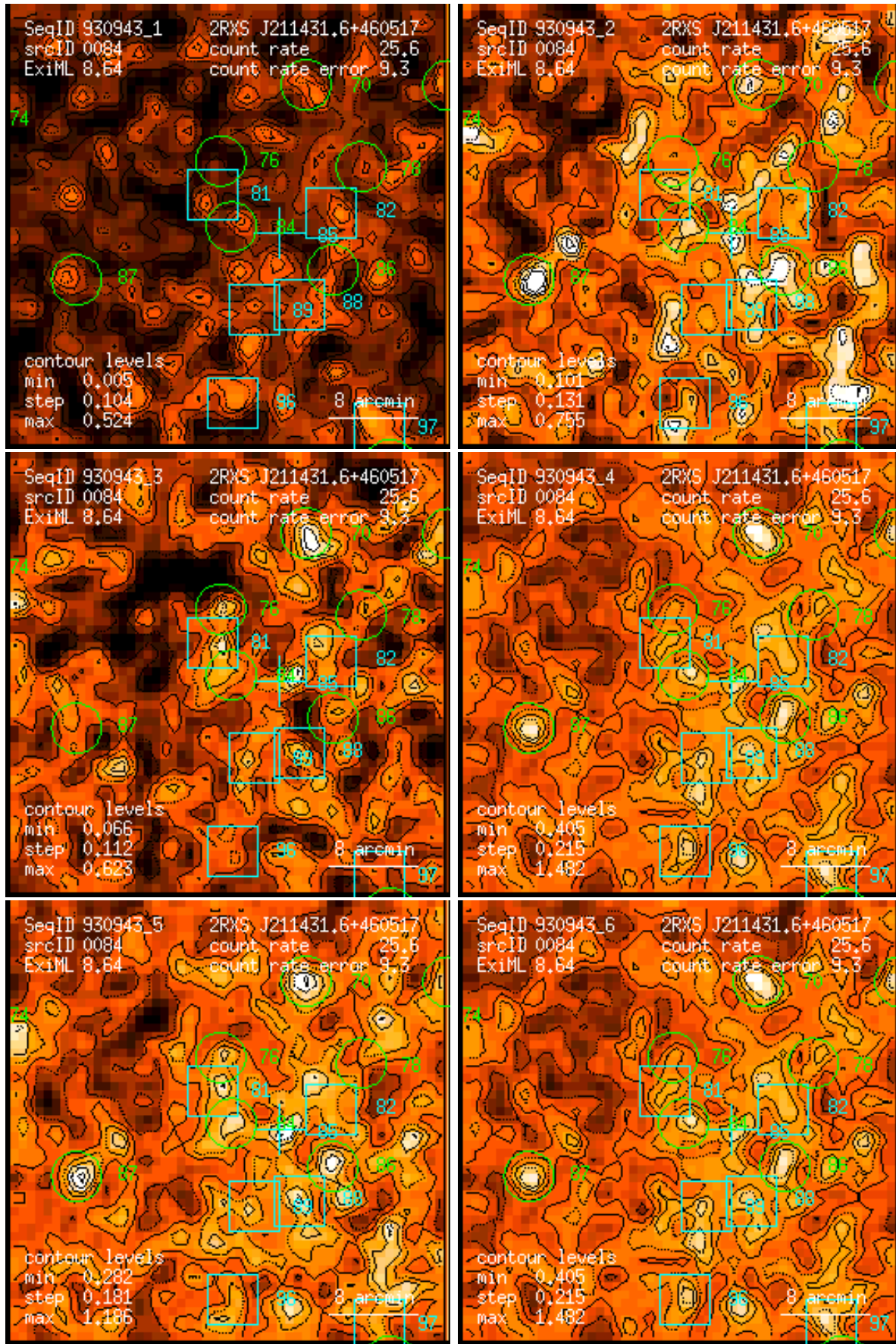
Figure 84: RASS 930943: detection 0084: band rate images, Gaussian filter: (1) PSPC channels 11 – 41, (2) 52 – 90, (3) 91 – 201, (4) 11 – 235, (5) 52 – 201, (6) 11 – 201. Broad band rates in counts/ks. Band rate contour levels in counts/ks/arcmin 2 .
