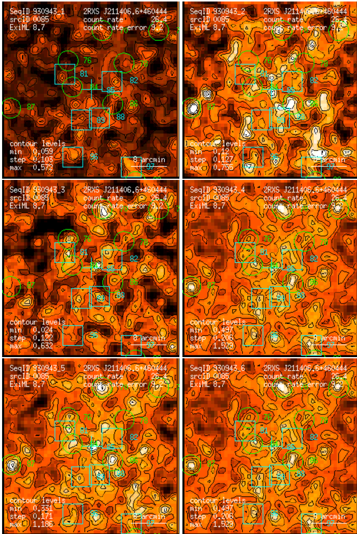
Figure 85: RASS 930943: detection 0085: band rate images, Gaussian filter: (1) PSPC channels 11 – 41, (2) 52 – 90, (3) 91 – 201, (4) 11 – 235, (5) 52 – 201, (6) 11 – 201. Broad band rates in counts/ks. Band rate contour levels in counts/ks/arcmin 2 .
