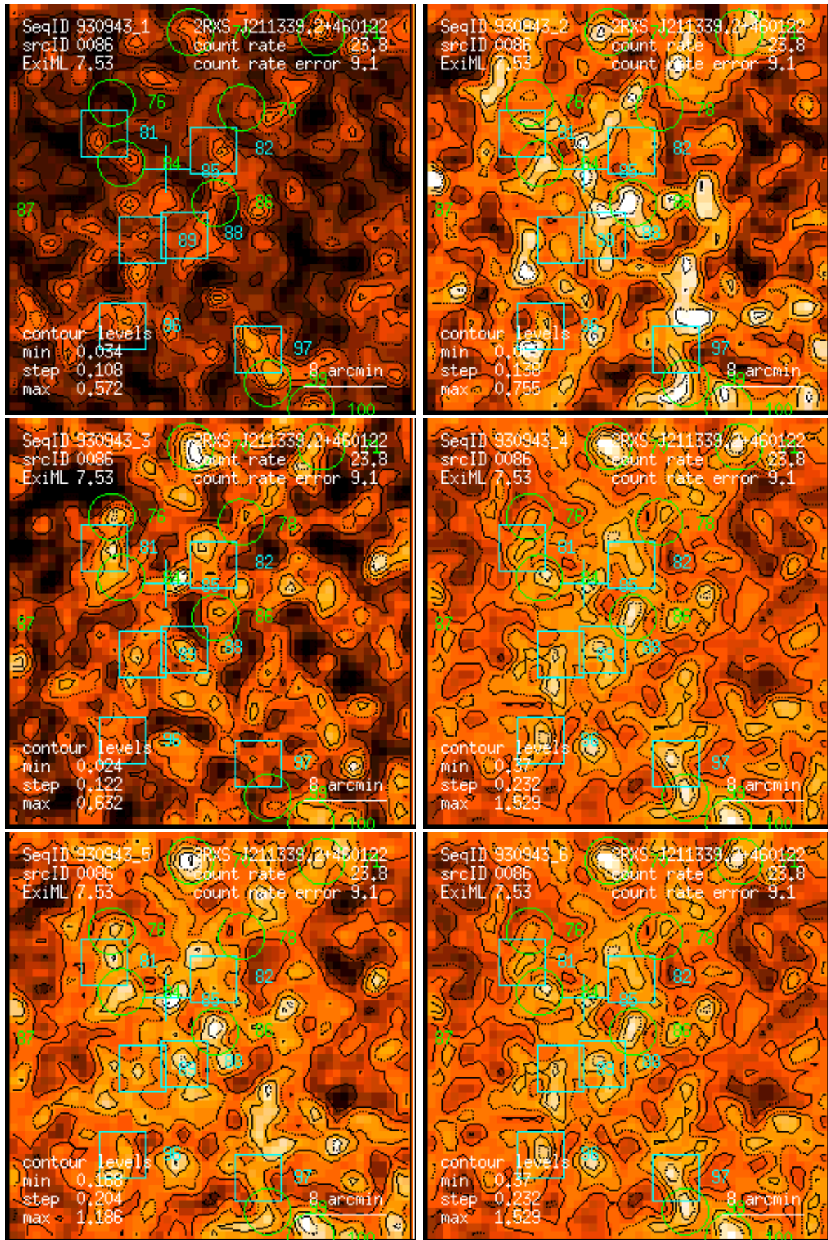
Figure 86: RASS 930943: detection 0086: band rate images, Gaussian filter: (1) PSPC channels 11 – 41, (2) 52 – 90, (3) 91 – 201, (4) 11 – 235, (5) 52 – 201, (6) 11 – 201. Broad band rates in counts/ks. Band rate contour levels in counts/ks/arcmin 2 .
