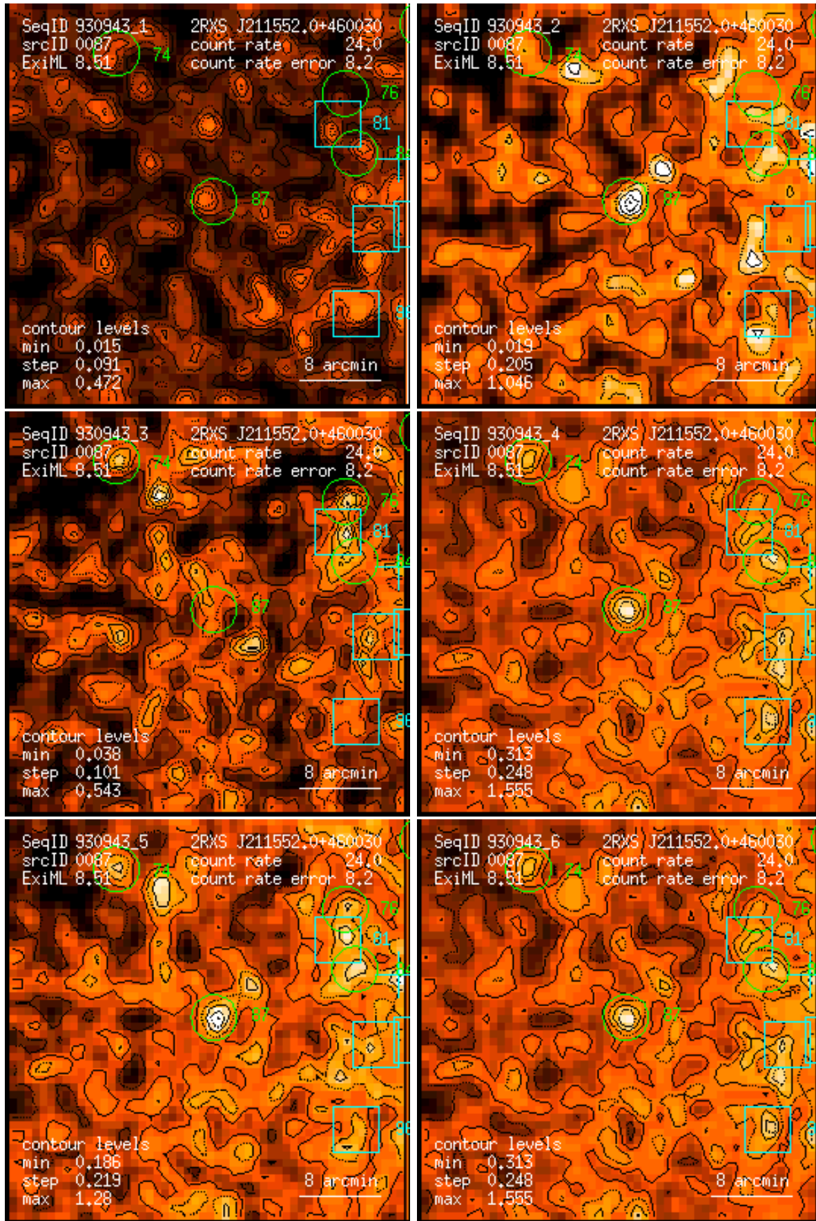
Figure 87: RASS 930943: detection 0087: band rate images, Gaussian filter: (1) PSPC channels 11 – 41, (2) 52 – 90, (3) 91 – 201, (4) 11 – 235, (5) 52 – 201, (6) 11 – 201. Broad band rates in counts/ks. Band rate contour levels in counts/ks/arcmin 2 .
