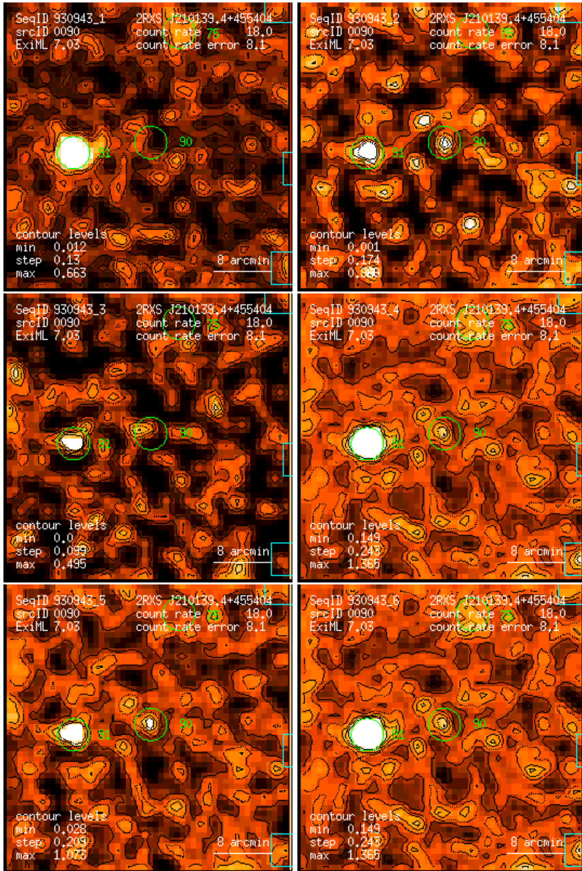
Figure 90: RASS 930943: detection 0090: band rate images, Gaussian filter: (1) PSPC channels 11 – 41, (2) 52 – 90, (3) 91 – 201, (4) 11 – 235, (5) 52 – 201, (6) 11 – 201. Broad band rates in counts/ks. Band rate contour levels in counts/ks/arcmin 2 .
