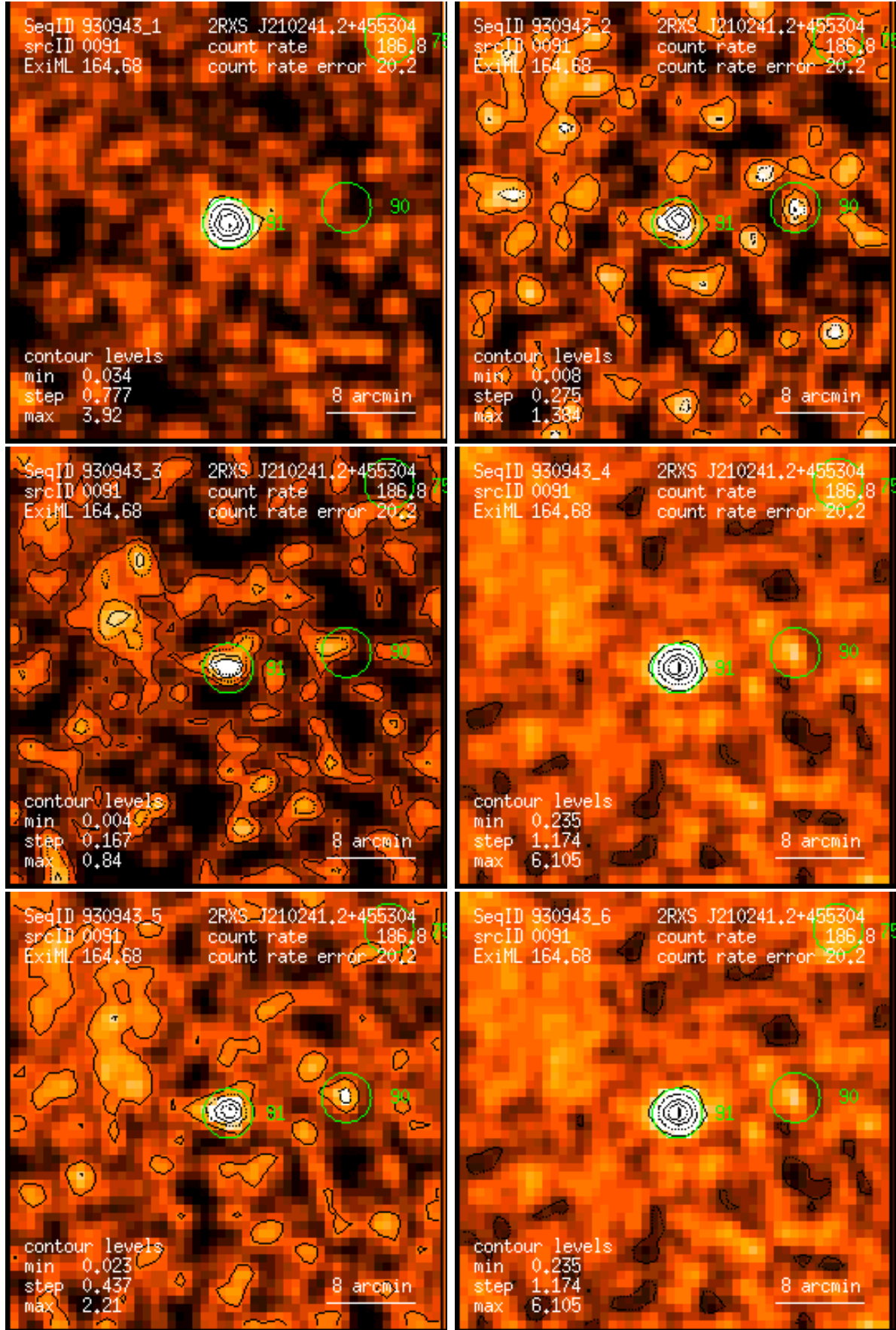
Figure 91: RASS 930943: detection 0091: band rate images, Gaussian filter: (1) PSPC channels 11 – 41, (2) 52 – 90, (3) 91 – 201, (4) 11 – 235, (5) 52 – 201, (6) 11 – 201. Broad band rates in counts/ks. Band rate contour levels in counts/ks/arcmin 2 .
