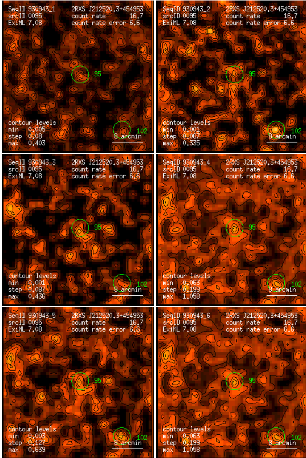
Figure 95: RASS 930943: detection 0095: band rate images, Gaussian filter: (1) PSPC channels 11 – 41, (2) 52 – 90, (3) 91 – 201, (4) 11 – 235, (5) 52 – 201, (6) 11 – 201. Broad band rates in counts/ks. Band rate contour levels in counts/ks/arcmin 2 .
