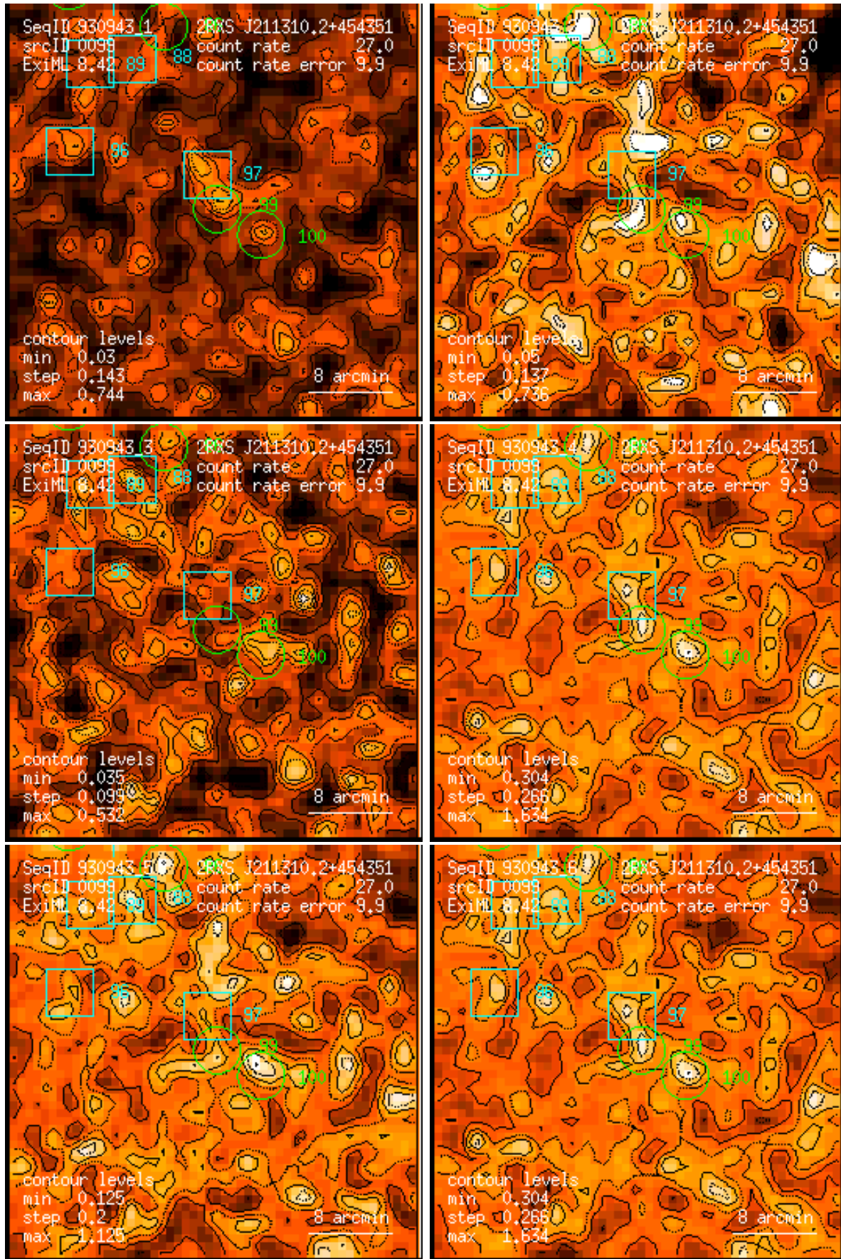
Figure 99: RASS 930943: detection 0099: band rate images, Gaussian filter: (1) PSPC channels 11 – 41, (2) 52 – 90, (3) 91 – 201, (4) 11 – 235, (5) 52 – 201, (6) 11 – 201. Broad band rates in counts/ks. Band rate contour levels in counts/ks/arcmin 2 .
