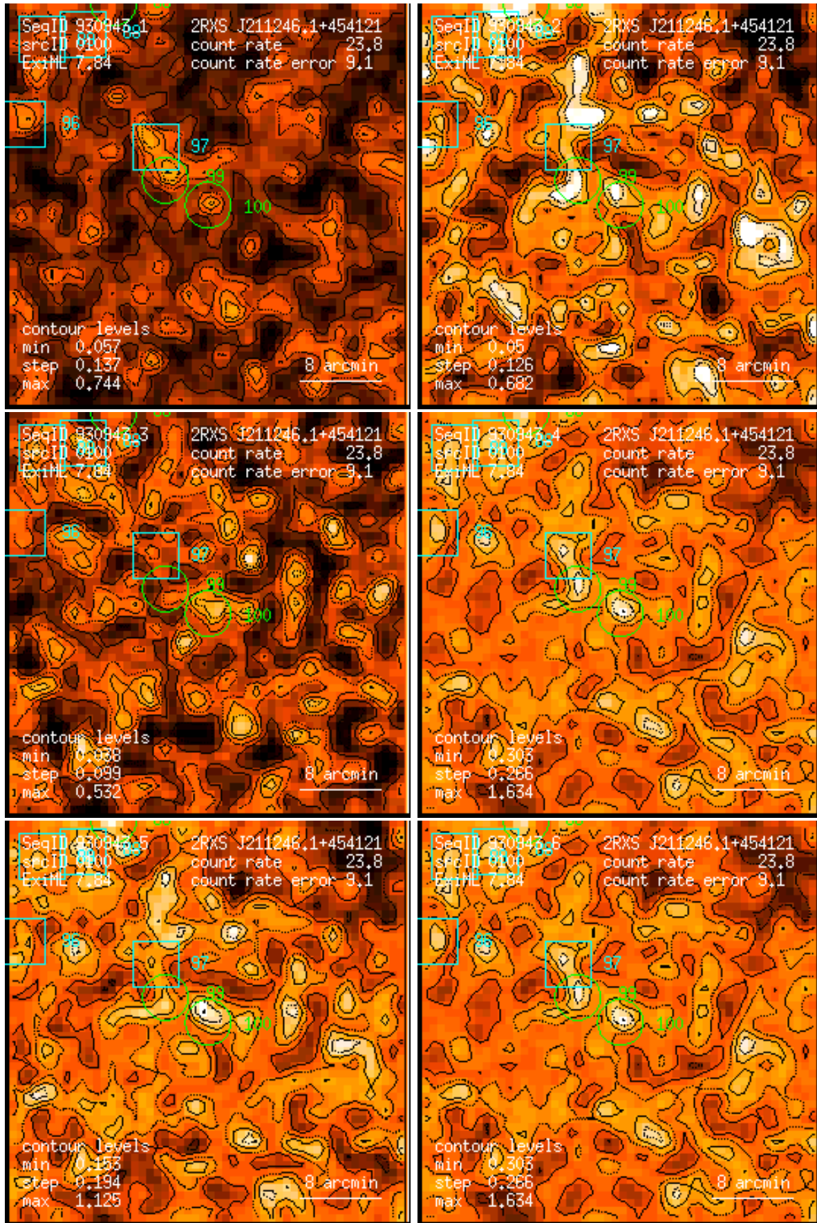
Figure 100: RASS 930943: detection 0100: band rate images, Gaussian filter: (1) PSPC channels 11 – 41, (2) 52 – 90, (3) 91 – 201, (4) 11 – 235, (5) 52 – 201, (6) 11 – 201. Broad band rates in counts/ks. Band rate contour levels in counts/ks/arcmin 2 .
