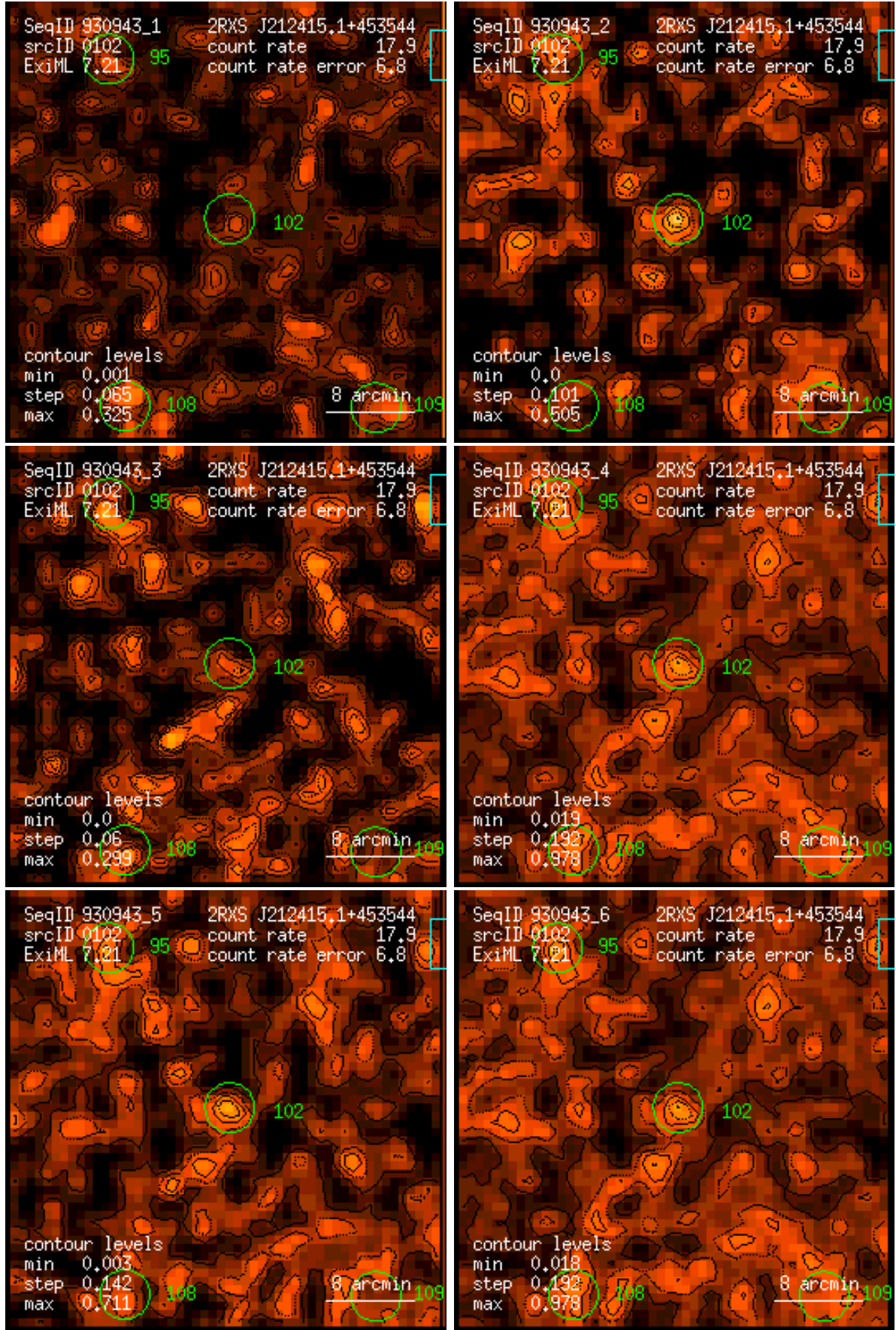
Figure 102: RASS 930943: detection 0102: band rate images, Gaussian filter: (1) PSPC channels 11 – 41, (2) 52 – 90, (3) 91 – 201, (4) 11 – 235, (5) 52 – 201, (6) 11 – 201. Broad band rates in counts/ks. Band rate contour levels in counts/ks/arcmin 2 .
