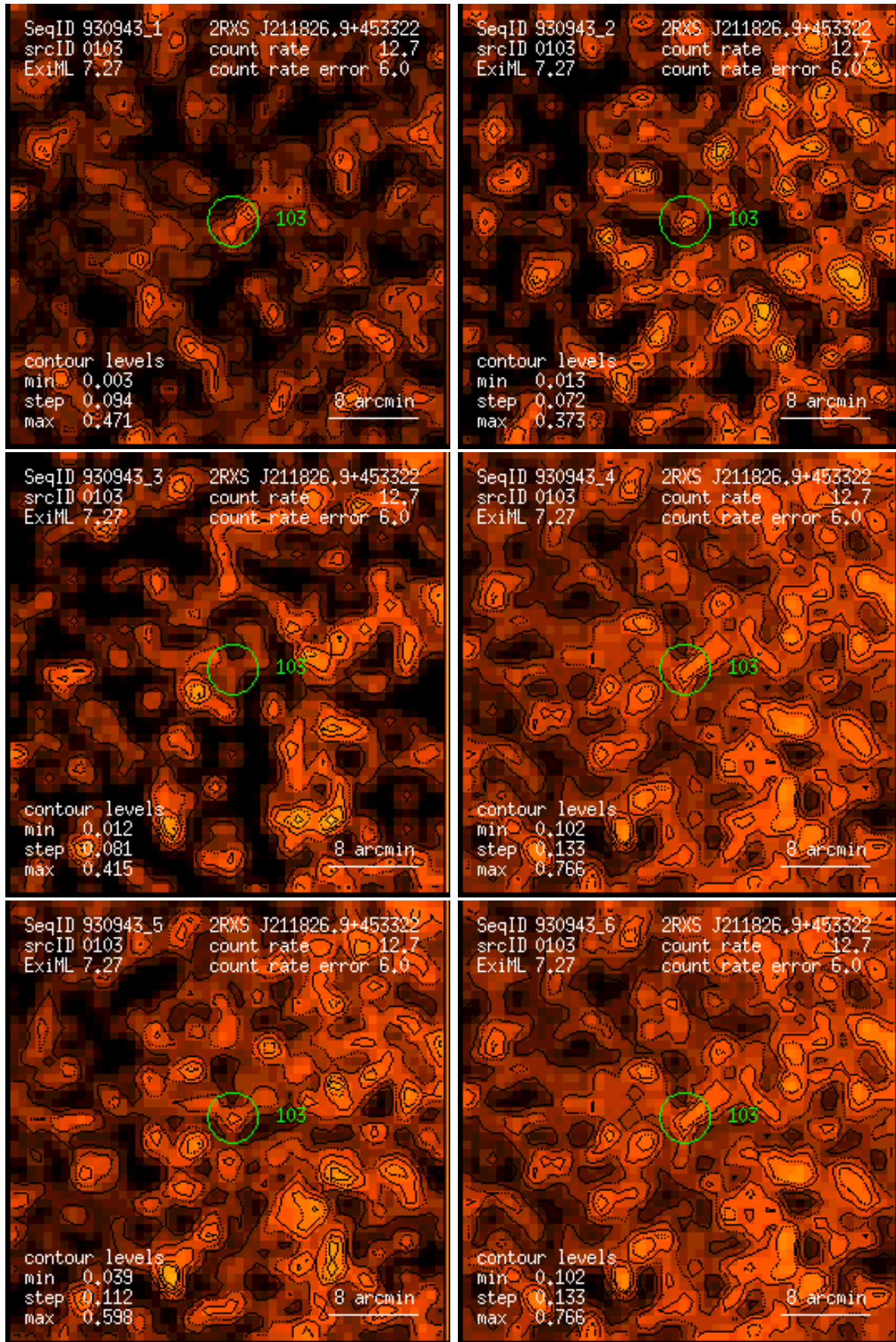
Figure 103: RASS 930943: detection 0103: band rate images, Gaussian filter: (1) PSPC channels 11 – 41, (2) 52 – 90, (3) 91 – 201, (4) 11 – 235, (5) 52 – 201, (6) 11 – 201. Broad band rates in counts/ks. Band rate contour levels in counts/ks/arcmin 2 .
