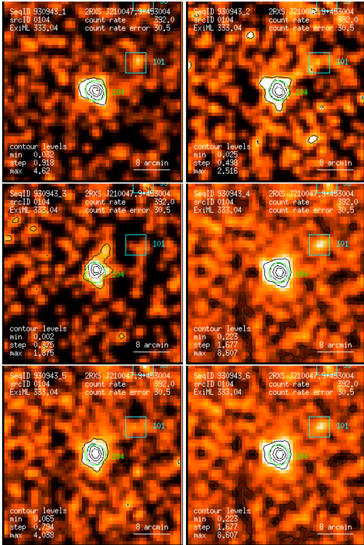
Figure 104: RASS 930943: detection 0104: band rate images, Gaussian filter: (1) PSPC channels 11 – 41, (2) 52 – 90, (3) 91 – 201, (4) 11 – 235, (5) 52 – 201, (6) 11 – 201. Broad band rates in counts/ks. Band rate contour levels in counts/ks/arcmin 2 .
