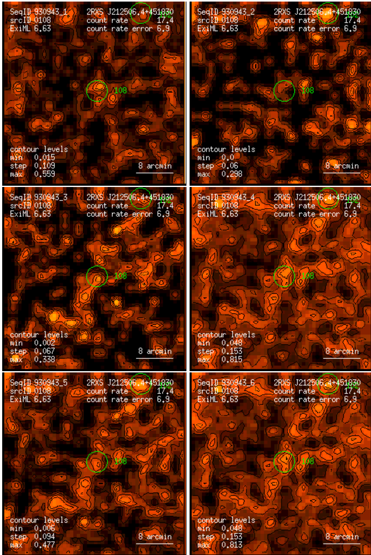
Figure 108: RASS 930943: detection 0108: band rate images, Gaussian filter: (1) PSPC channels 11 – 41, (2) 52 – 90, (3) 91 – 201, (4) 11 – 235, (5) 52 – 201, (6) 11 – 201. Broad band rates in counts/ks. Band rate contour levels in counts/ks/arcmin 2 .
