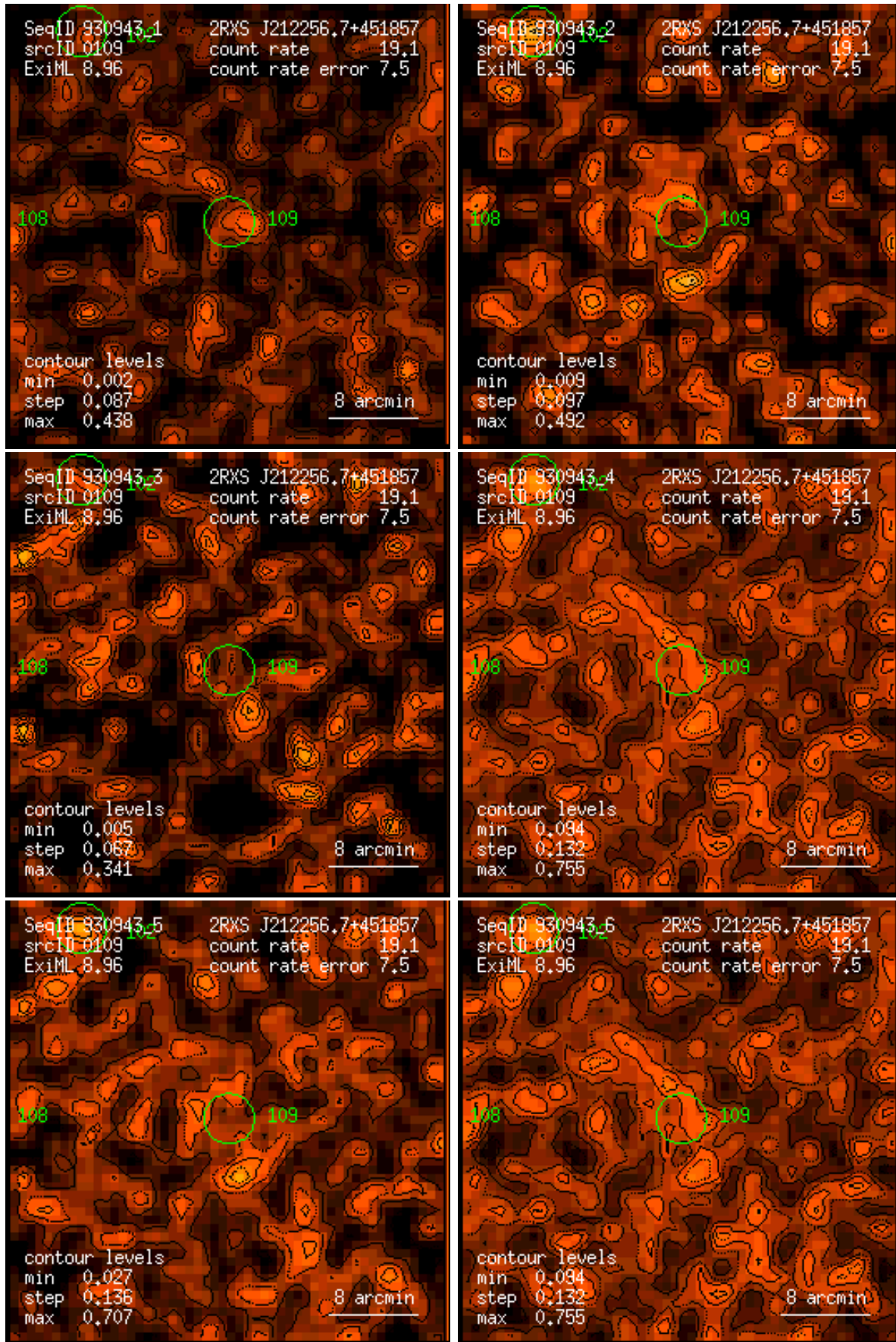
Figure 109: RASS 930943: detection 0109: band rate images, Gaussian filter: (1) PSPC channels 11 – 41, (2) 52 – 90, (3) 91 – 201, (4) 11 – 235, (5) 52 – 201, (6) 11 – 201. Broad band rates in counts/ks. Band rate contour levels in counts/ks/arcmin 2 .
