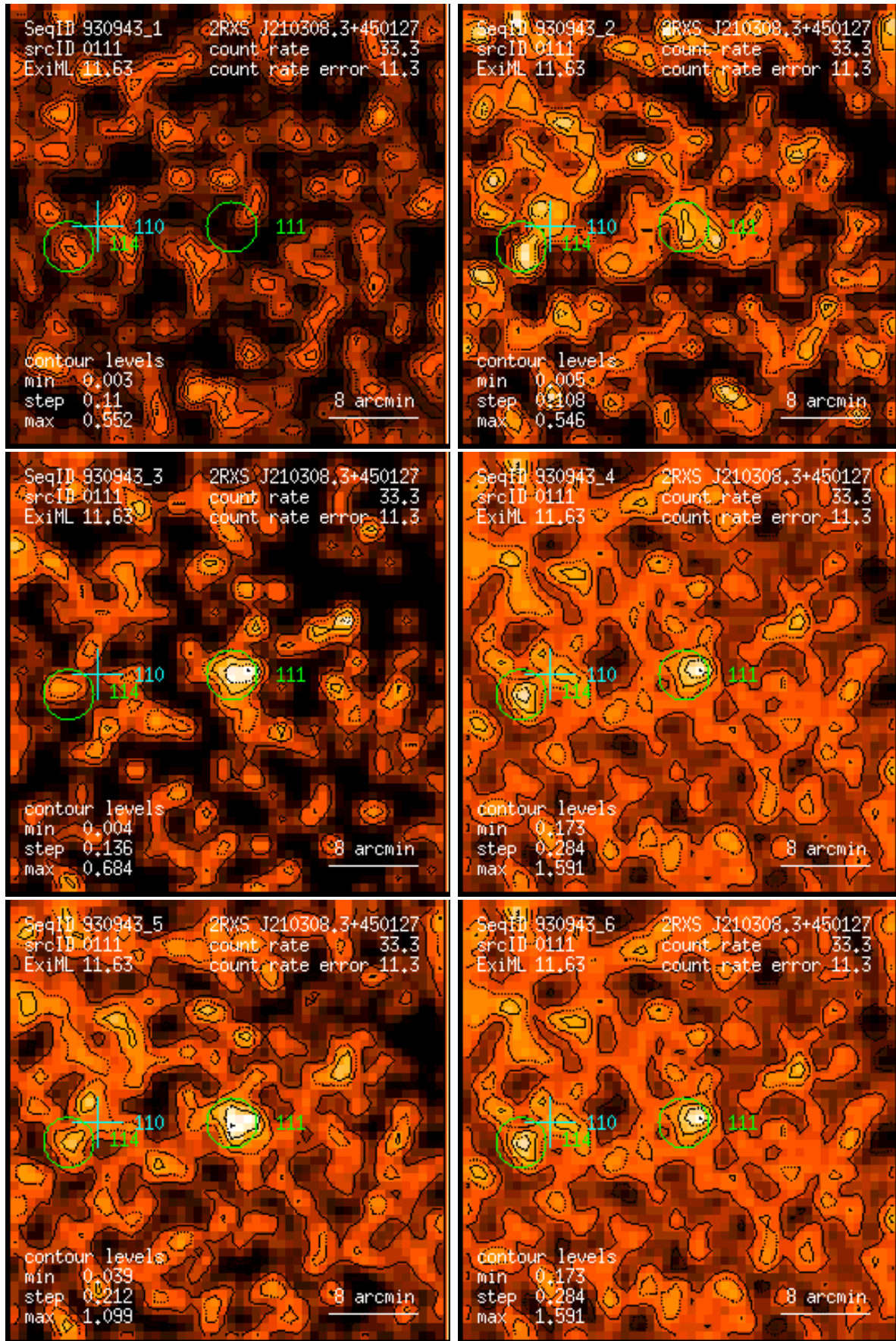
Figure 111: RASS 930943: detection 0111: band rate images, Gaussian filter: (1) PSPC channels 11 – 41, (2) 52 – 90, (3) 91 – 201, (4) 11 – 235, (5) 52 – 201, (6) 11 – 201. Broad band rates in counts/ks. Band rate contour levels in counts/ks/arcmin 2 .
