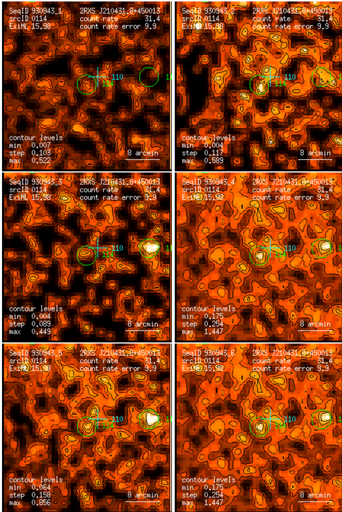
Figure 114: RASS 930943: detection 0114: band rate images, Gaussian filter: (1) PSPC channels 11 – 41, (2) 52 – 90, (3) 91 – 201, (4) 11 – 235, (5) 52 – 201, (6) 11 – 201. Broad band rates in counts/ks. Band rate contour levels in counts/ks/arcmin 2 .
