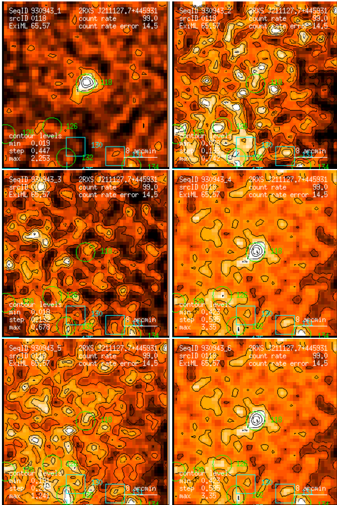
Figure 118: RASS 930943: detection 0118: band rate images, Gaussian filter: (1) PSPC channels 11 – 41, (2) 52 – 90, (3) 91 – 201, (4) 11 – 235, (5) 52 – 201, (6) 11 – 201. Broad band rates in counts/ks. Band rate contour levels in counts/ks/arcmin 2 .
