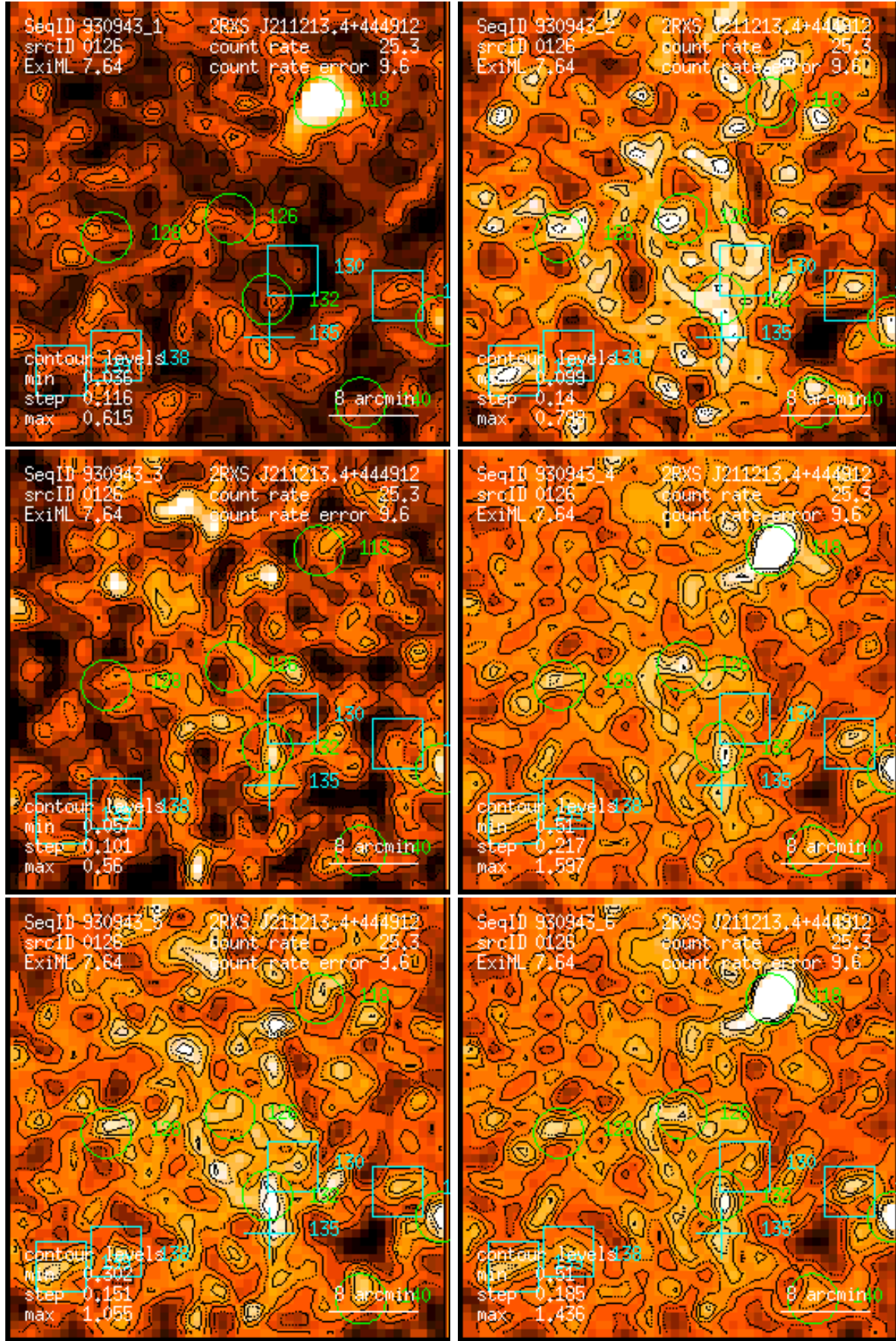
Figure 126: RASS 930943: detection 0126: band rate images, Gaussian filter: (1) PSPC channels 11 – 41, (2) 52 – 90, (3) 91 – 201, (4) 11 – 235, (5) 52 – 201, (6) 11 – 201. Broad band rates in counts/ks. Band rate contour levels in counts/ks/arcmin 2 .
