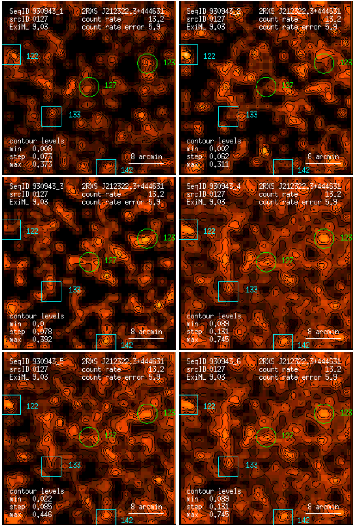
Figure 127: RASS 930943: detection 0127: band rate images, Gaussian filter: (1) PSPC channels 11 – 41, (2) 52 – 90, (3) 91 – 201, (4) 11 – 235, (5) 52 – 201, (6) 11 – 201. Broad band rates in counts/ks. Band rate contour levels in counts/ks/arcmin 2 .
