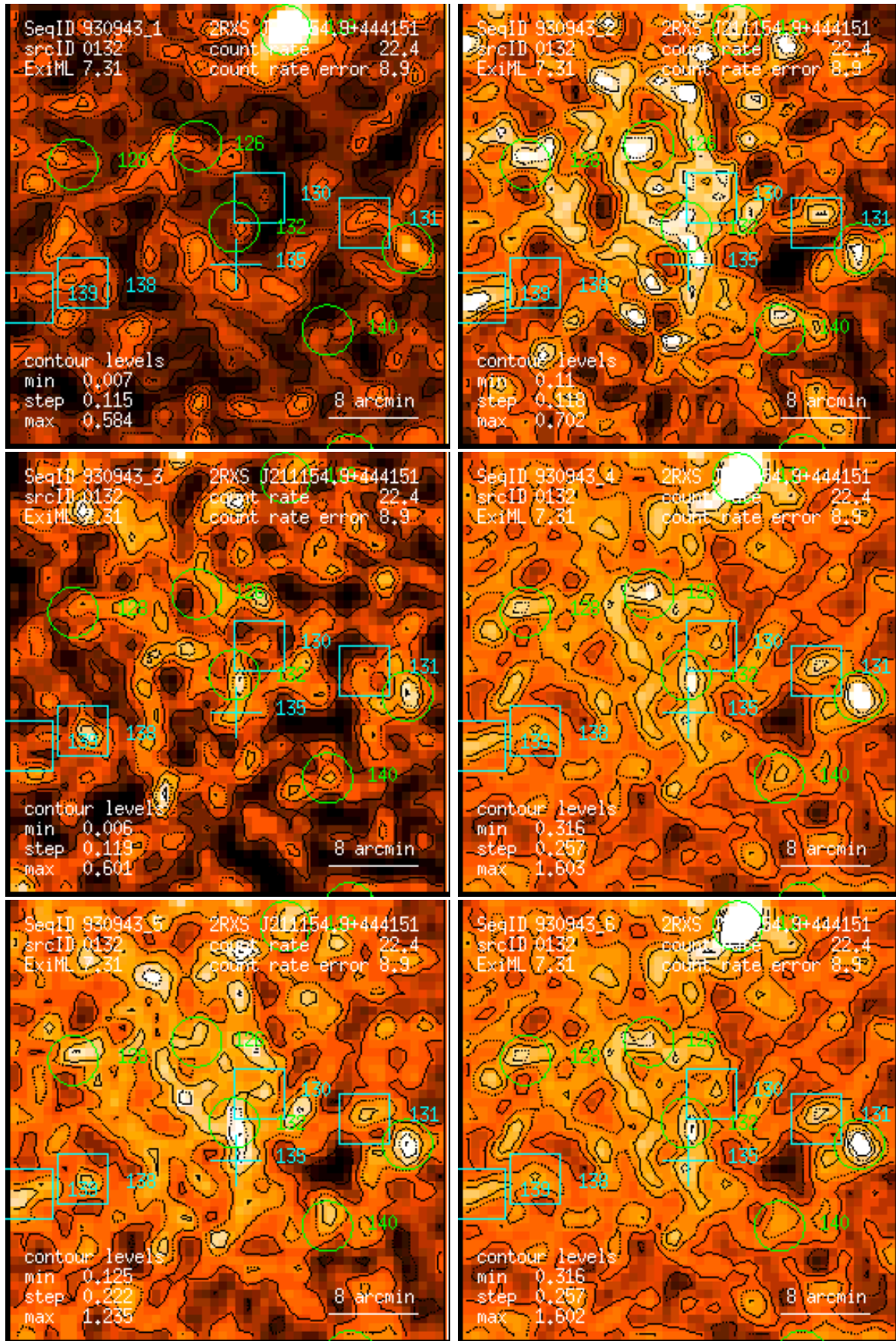
Figure 132: RASS 930943: detection 0132: band rate images, Gaussian filter: (1) PSPC channels 11 – 41, (2) 52 – 90, (3) 91 – 201, (4) 11 – 235, (5) 52 – 201, (6) 11 – 201. Broad band rates in counts/ks. Band rate contour levels in counts/ks/arcmin 2 .
