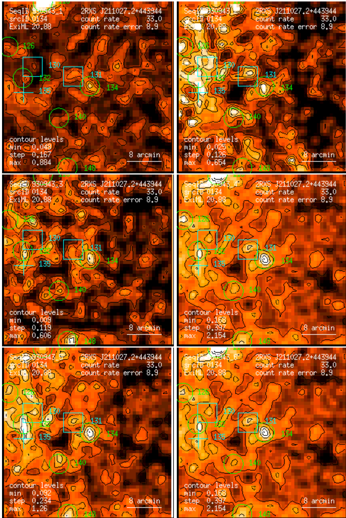
Figure 134: RASS 930943: detection 0134: band rate images, Gaussian filter: (1) PSPC channels 11 – 41, (2) 52 – 90, (3) 91 – 201, (4) 11 – 235, (5) 52 – 201, (6) 11 – 201. Broad band rates in counts/ks. Band rate contour levels in counts/ks/arcmin 2 .
