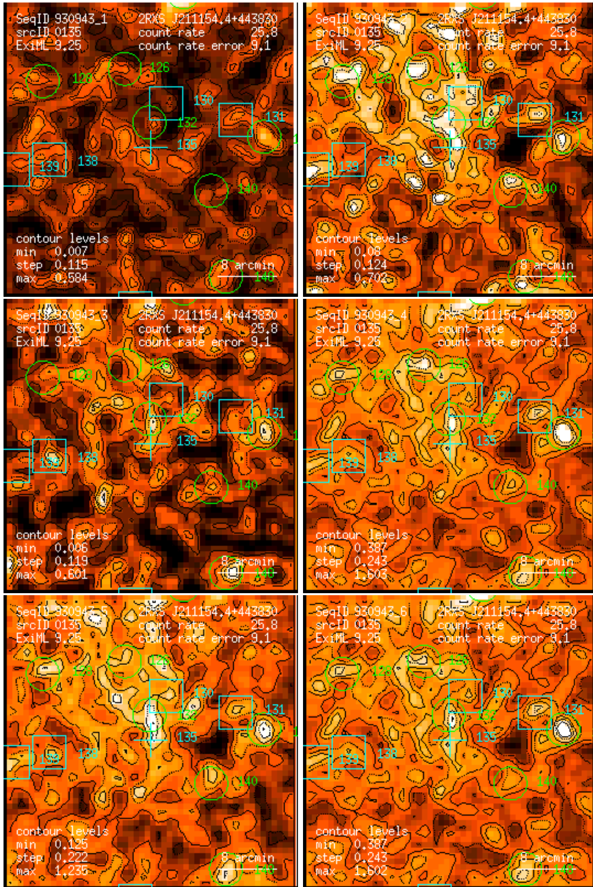
Figure 135: RASS 930943: detection 0135: band rate images, Gaussian filter: (1) PSPC channels 11 – 41, (2) 52 – 90, (3) 91 – 201, (4) 11 – 235, (5) 52 – 201, (6) 11 – 201. Broad band rates in counts/ks. Band rate contour levels in counts/ks/arcmin 2 .
