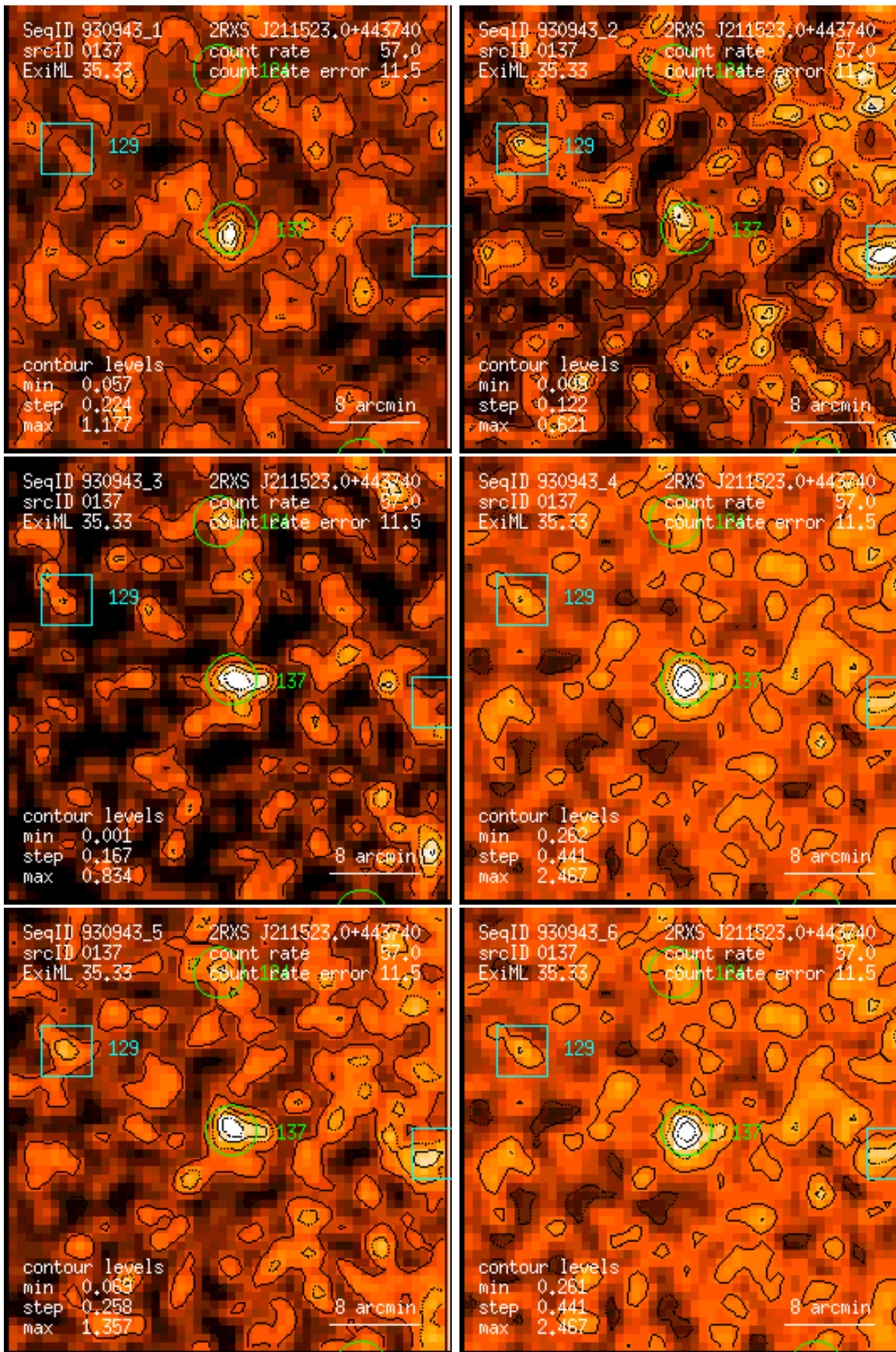
Figure 137: RASS 930943: detection 0137: band rate images, Gaussian filter: (1) PSPC channels 11 – 41, (2) 52 – 90, (3) 91 – 201, (4) 11 – 235, (5) 52 – 201, (6) 11 – 201. Broad band rates in counts/ks. Band rate contour levels in counts/ks/arcmin 2 .
