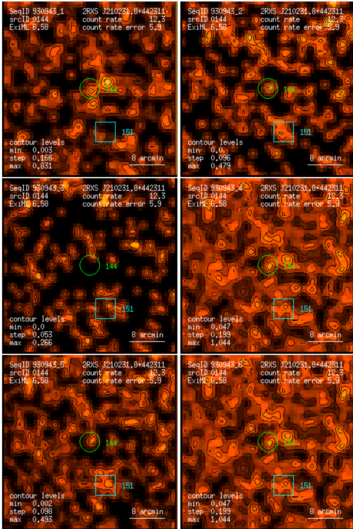
Figure 144: RASS 930943: detection 0144: band rate images, Gaussian filter: (1) PSPC channels 11 – 41, (2) 52 – 90, (3) 91 – 201, (4) 11 – 235, (5) 52 – 201, (6) 11 – 201. Broad band rates in counts/ks. Band rate contour levels in counts/ks/arcmin 2 .
