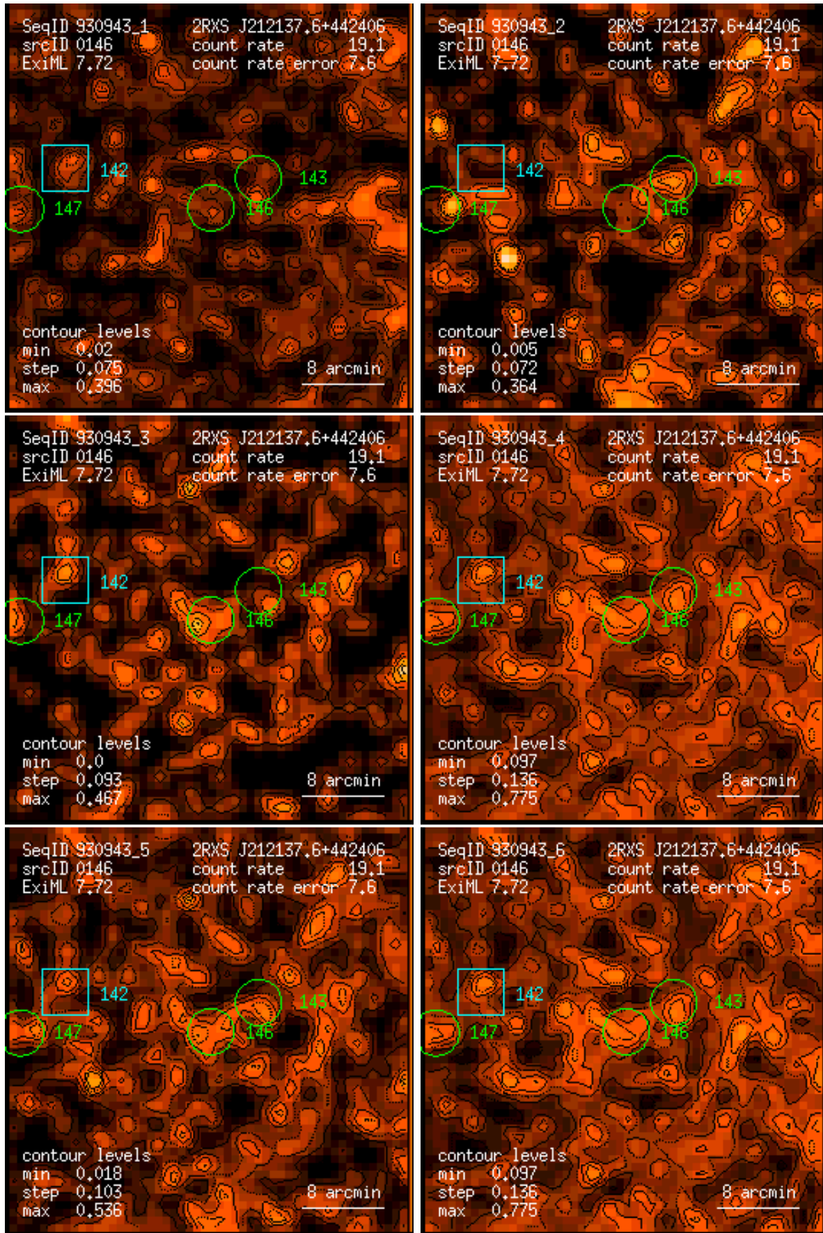
Figure 146: RASS 930943: detection 0146: band rate images, Gaussian filter: (1) PSPC channels 11 – 41, (2) 52 – 90, (3) 91 – 201, (4) 11 – 235, (5) 52 – 201, (6) 11 – 201. Broad band rates in counts/ks. Band rate contour levels in counts/ks/arcmin 2 .
