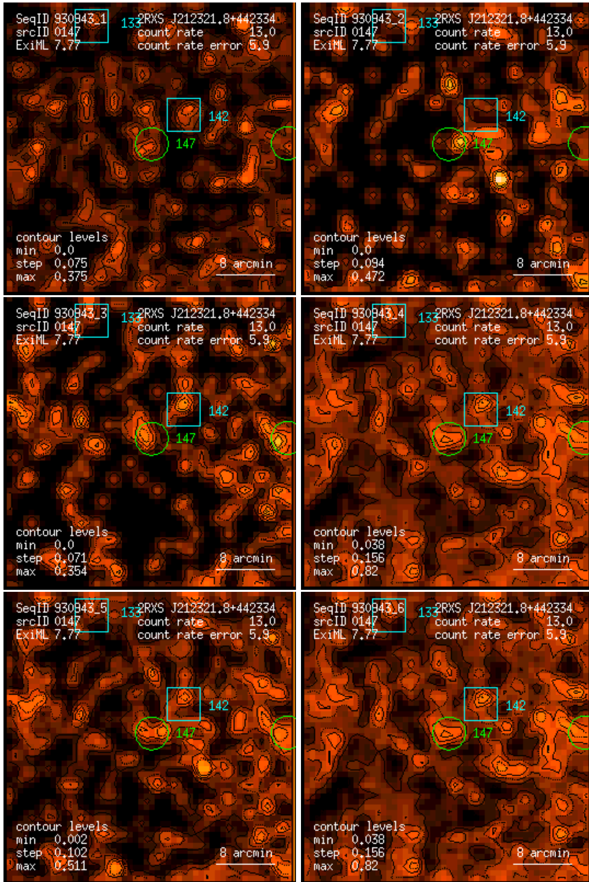
Figure 147: RASS 930943: detection 0147: band rate images, Gaussian filter: (1) PSPC channels 11 – 41, (2) 52 – 90, (3) 91 – 201, (4) 11 – 235, (5) 52 – 201, (6) 11 – 201. Broad band rates in counts/ks. Band rate contour levels in counts/ks/arcmin 2 .
