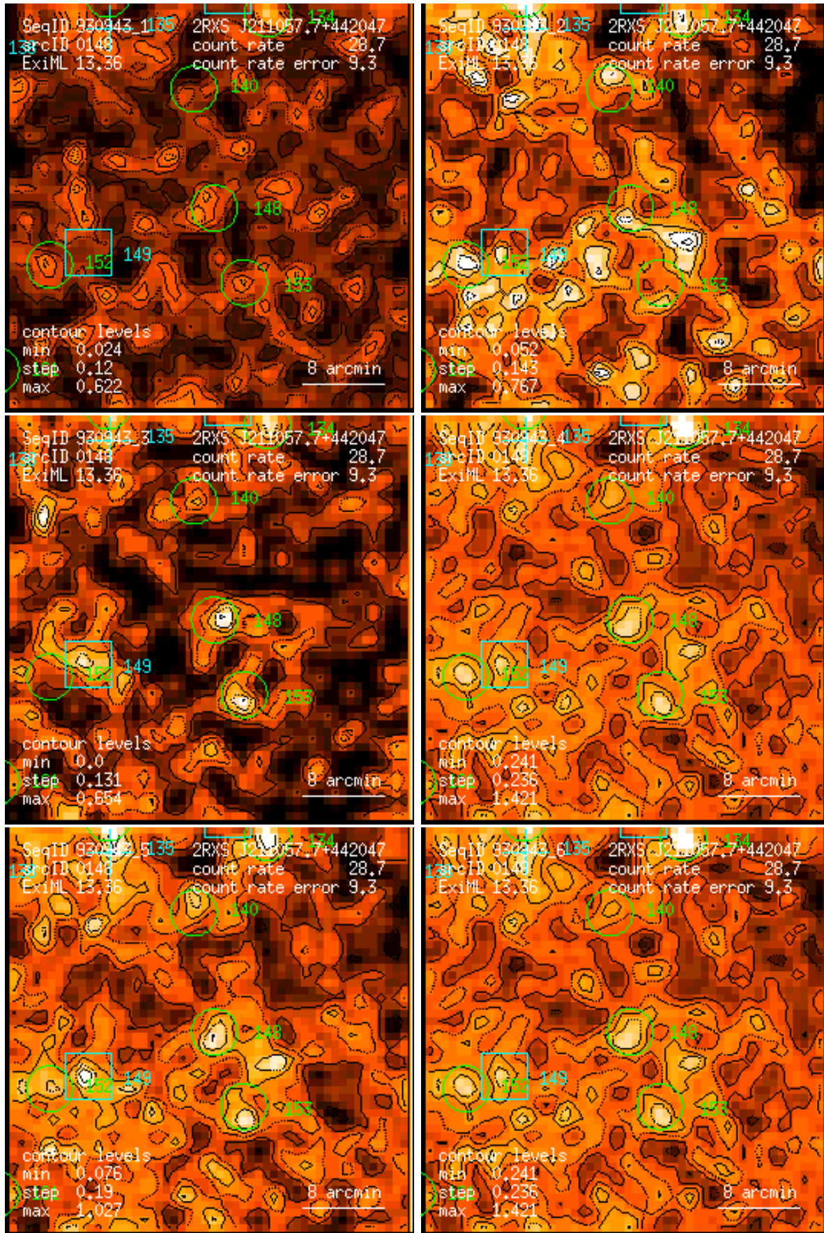
Figure 148: RASS 930943: detection 0148: band rate images, Gaussian filter: (1) PSPC channels 11 – 41, (2) 52 – 90, (3) 91 – 201, (4) 11 – 235, (5) 52 – 201, (6) 11 – 201. Broad band rates in counts/ks. Band rate contour levels in counts/ks/arcmin 2 .
