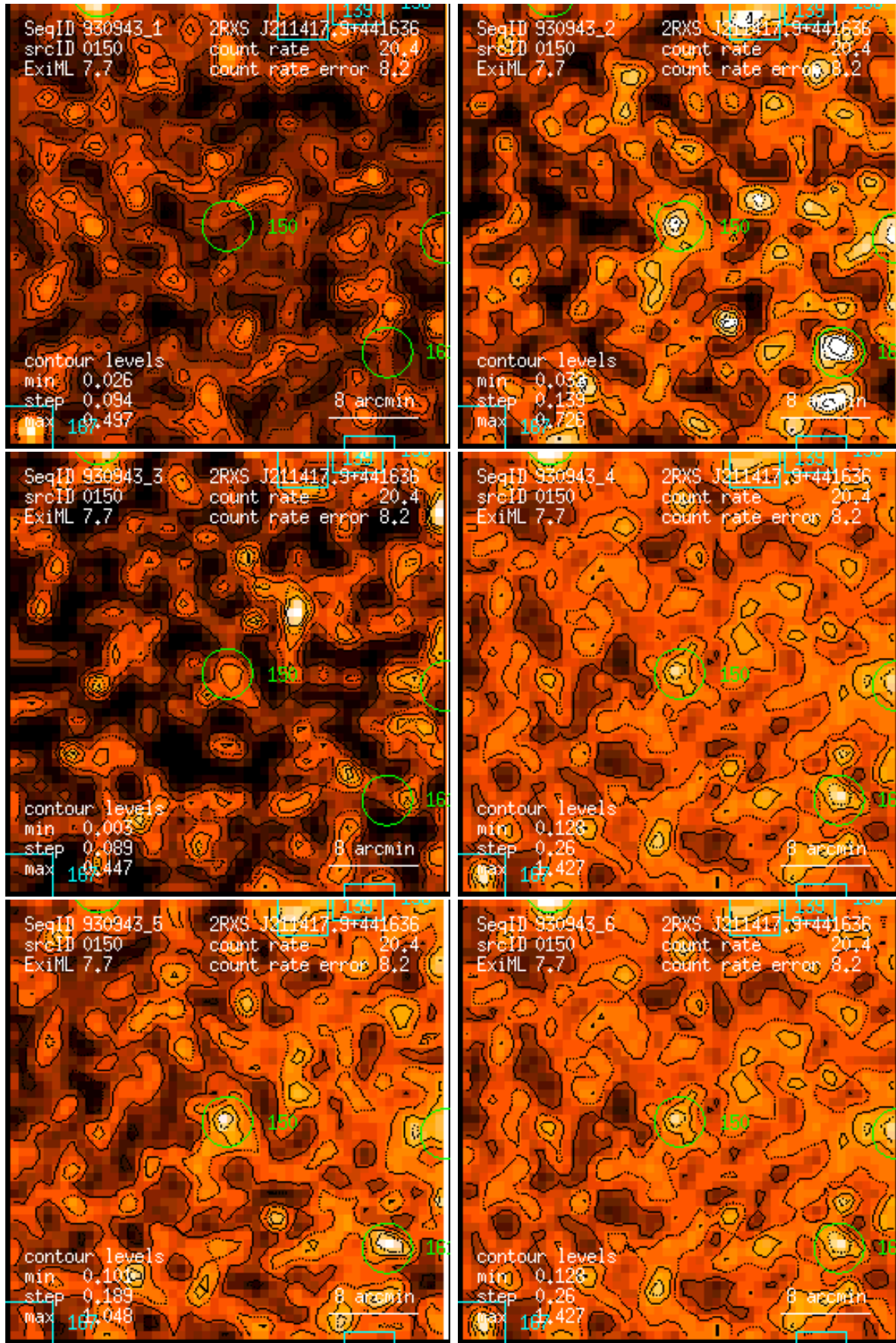
Figure 150: RASS 930943: detection 0150: band rate images, Gaussian filter: (1) PSPC channels 11 – 41, (2) 52 – 90, (3) 91 – 201, (4) 11 – 235, (5) 52 – 201, (6) 11 – 201. Broad band rates in counts/ks. Band rate contour levels in counts/ks/arcmin 2 .
