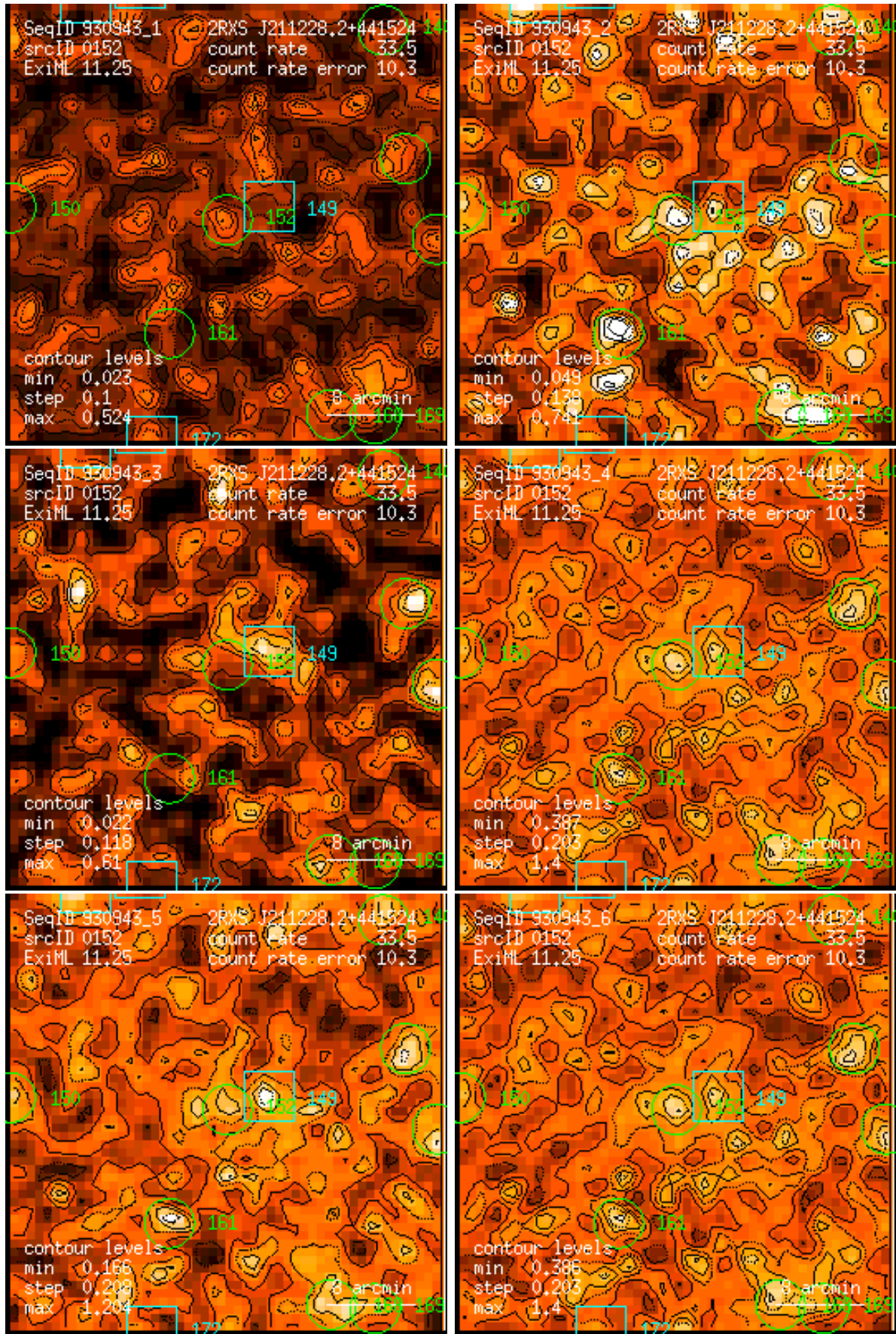
Figure 152: RASS 930943: detection 0152: band rate images, Gaussian filter: (1) PSPC channels 11 – 41, (2) 52 – 90, (3) 91 – 201, (4) 11 – 235, (5) 52 – 201, (6) 11 – 201. Broad band rates in counts/ks. Band rate contour levels in counts/ks/arcmin 2 .
