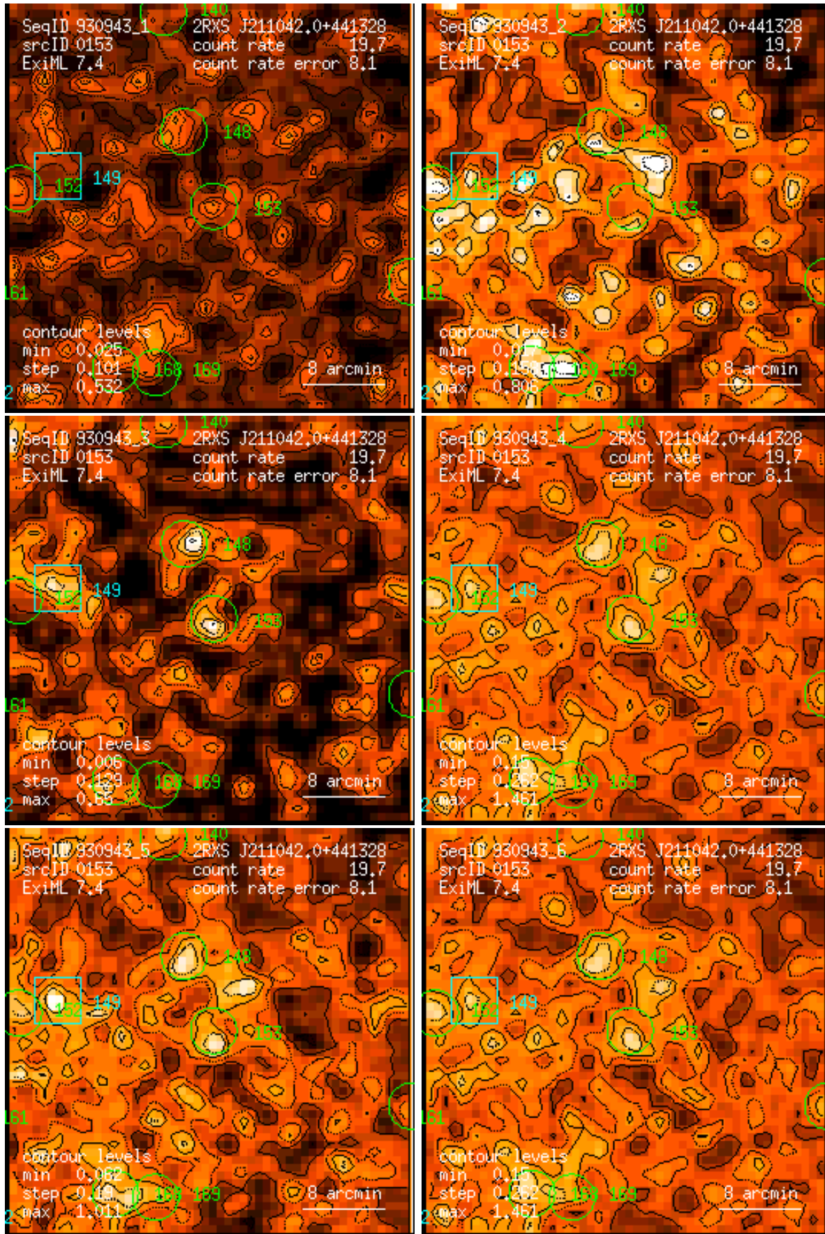
Figure 153: RASS 930943: detection 0153: band rate images, Gaussian filter: (1) PSPC channels 11 – 41, (2) 52 – 90, (3) 91 – 201, (4) 11 – 235, (5) 52 – 201, (6) 11 – 201. Broad band rates in counts/ks. Band rate contour levels in counts/ks/arcmin 2 .
