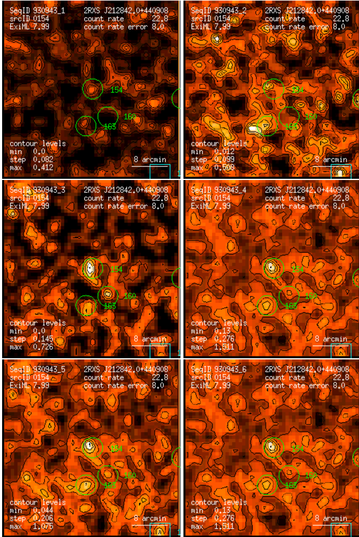
Figure 154: RASS 930943: detection 0154: band rate images, Gaussian filter: (1) PSPC channels 11 – 41, (2) 52 – 90, (3) 91 – 201, (4) 11 – 235, (5) 52 – 201, (6) 11 – 201. Broad band rates in counts/ks. Band rate contour levels in counts/ks/arcmin 2 .
