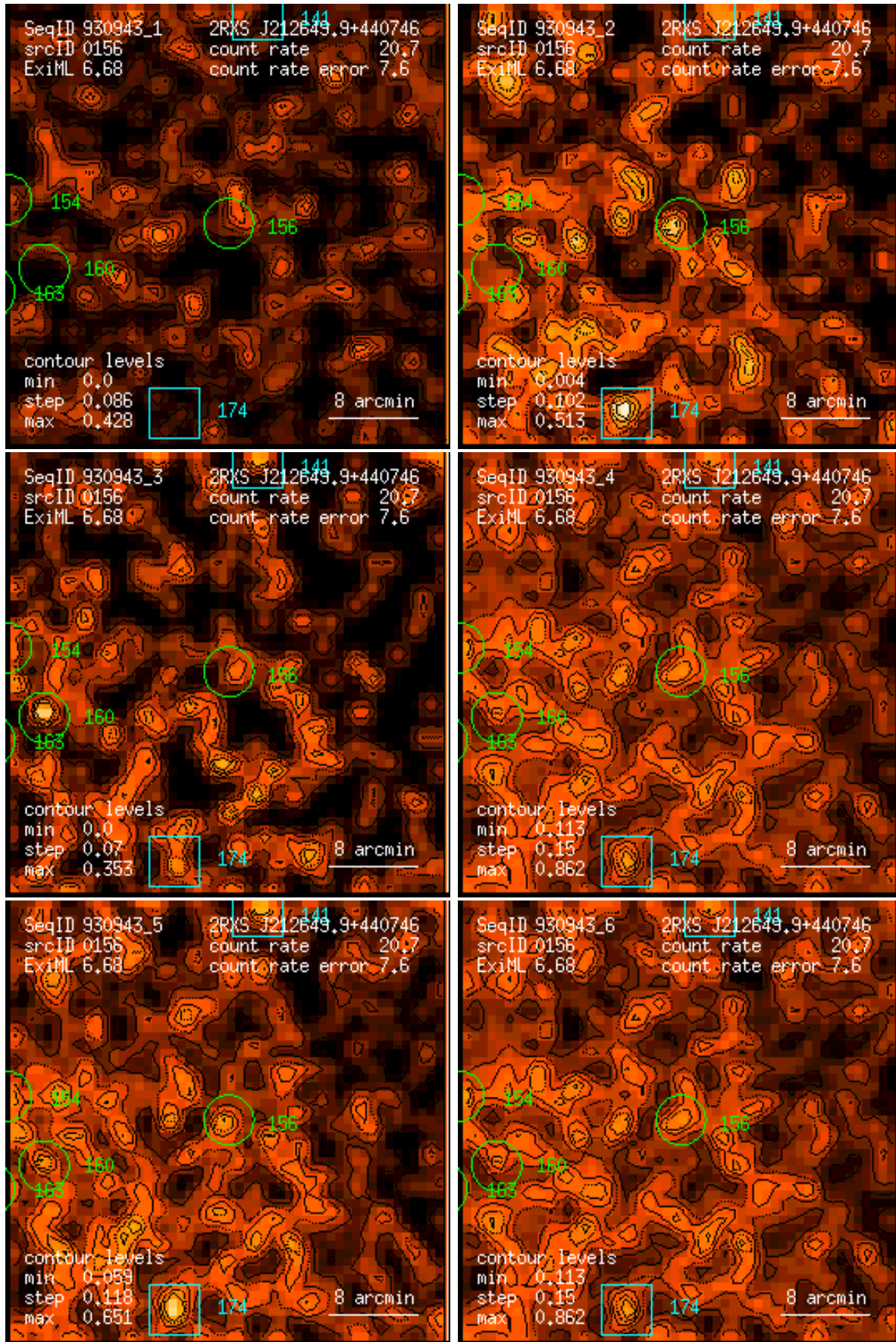
Figure 156: RASS 930943: detection 0156: band rate images, Gaussian filter: (1) PSPC channels 11 – 41, (2) 52 – 90, (3) 91 – 201, (4) 11 – 235, (5) 52 – 201, (6) 11 – 201. Broad band rates in counts/ks. Band rate contour levels in counts/ks/arcmin 2 .
