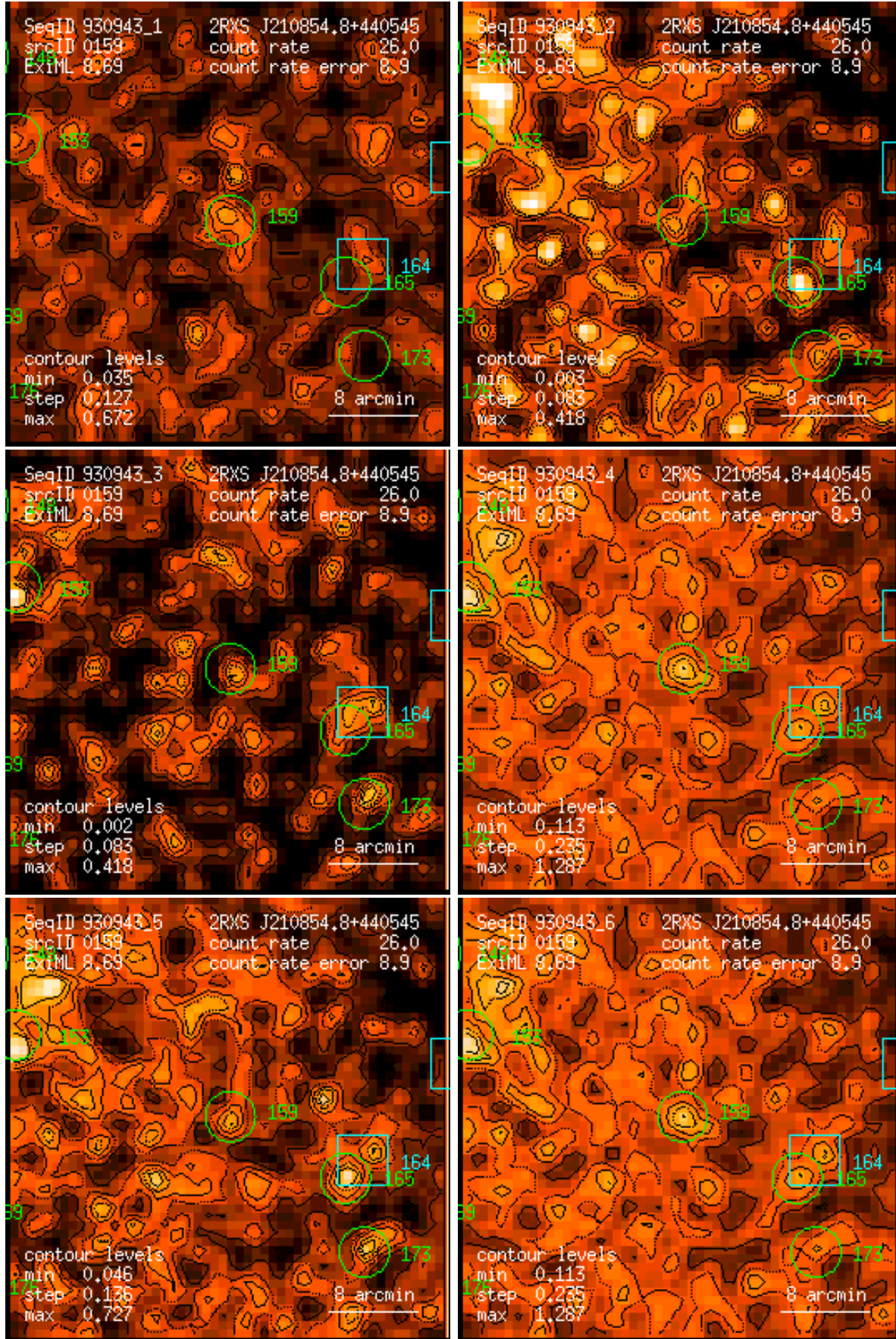
Figure 159: RASS 930943: detection 0159: band rate images, Gaussian filter: (1) PSPC channels 11 – 41, (2) 52 – 90, (3) 91 – 201, (4) 11 – 235, (5) 52 – 201, (6) 11 – 201. Broad band rates in counts/ks. Band rate contour levels in counts/ks/arcmin 2 .
