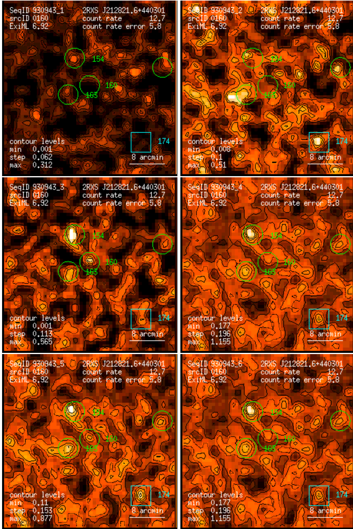
Figure 160: RASS 930943: detection 0160: band rate images, Gaussian filter: (1) PSPC channels 11 – 41, (2) 52 – 90, (3) 91 – 201, (4) 11 – 235, (5) 52 – 201, (6) 11 – 201. Broad band rates in counts/ks. Band rate contour levels in counts/ks/arcmin 2 .
