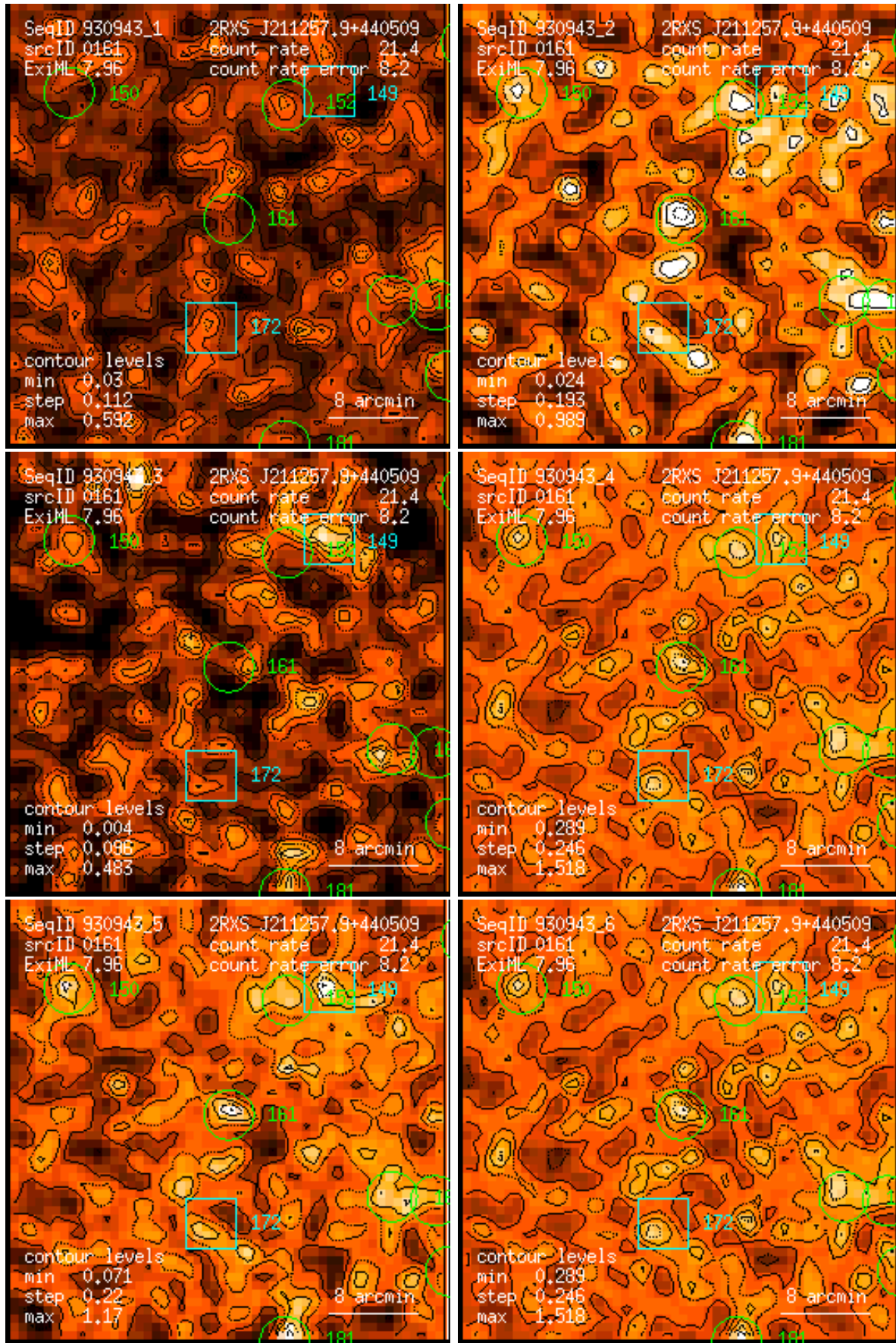
Figure 161: RASS 930943: detection 0161: band rate images, Gaussian filter: (1) PSPC channels 11 – 41, (2) 52 – 90, (3) 91 – 201, (4) 11 – 235, (5) 52 – 201, (6) 11 – 201. Broad band rates in counts/ks. Band rate contour levels in counts/ks/arcmin 2 .
