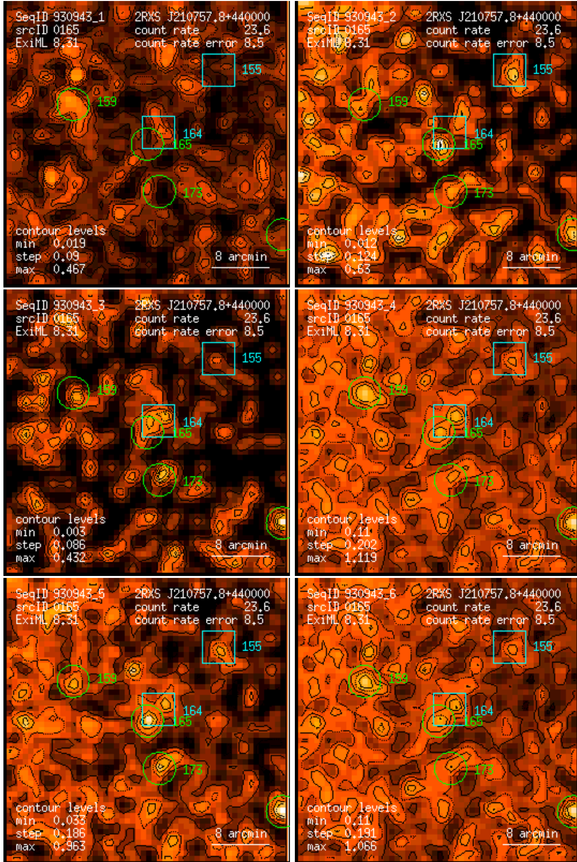
Figure 165: RASS 930943: detection 0165: band rate images, Gaussian filter: (1) PSPC channels 11 – 41, (2) 52 – 90, (3) 91 – 201, (4) 11 – 235, (5) 52 – 201, (6) 11 – 201. Broad band rates in counts/ks. Band rate contour levels in counts/ks/arcmin 2 .
