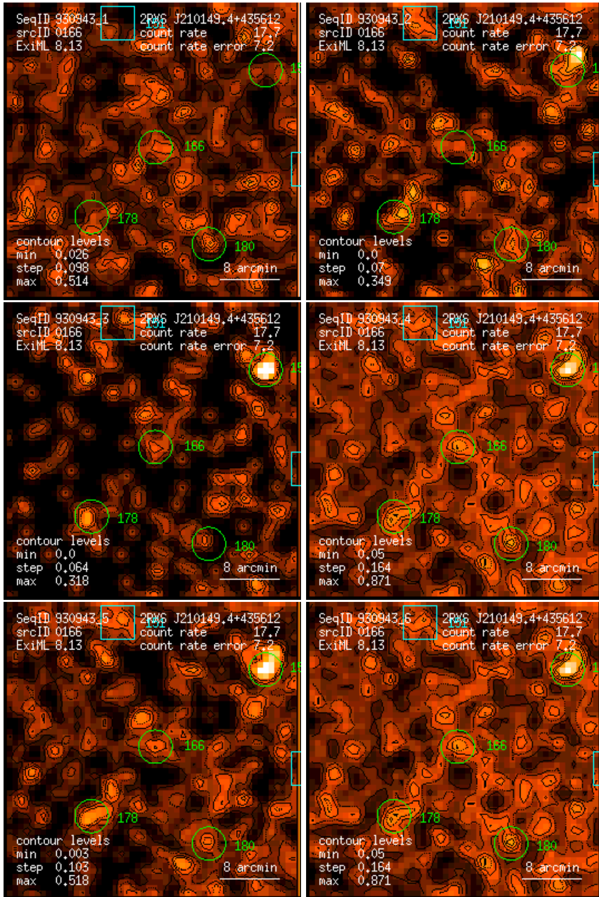
Figure 166: RASS 930943: detection 0166: band rate images, Gaussian filter: (1) PSPC channels 11 – 41, (2) 52 – 90, (3) 91 – 201, (4) 11 – 235, (5) 52 – 201, (6) 11 – 201. Broad band rates in counts/ks. Band rate contour levels in counts/ks/arcmin 2 .
