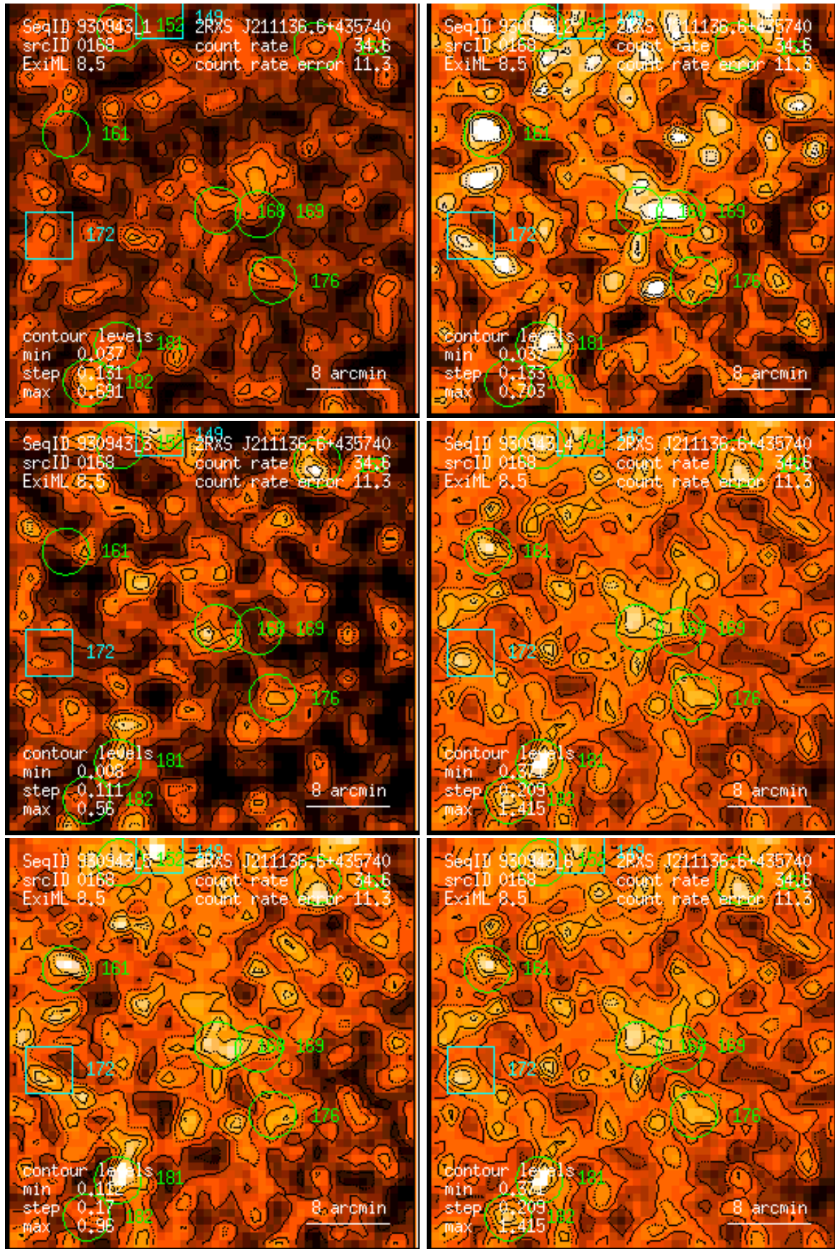
Figure 168: RASS 930943: detection 0168: band rate images, Gaussian filter: (1) PSPC channels 11 – 41, (2) 52 – 90, (3) 91 – 201, (4) 11 – 235, (5) 52 – 201, (6) 11 – 201. Broad band rates in counts/ks. Band rate contour levels in counts/ks/arcmin 2 .
