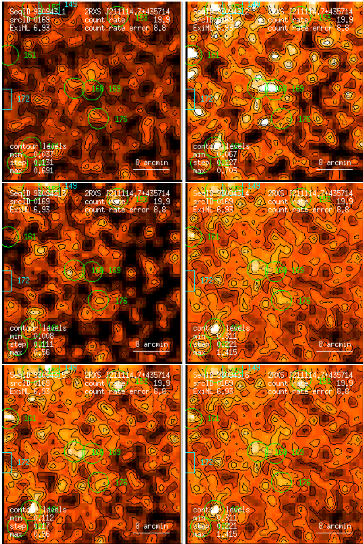
Figure 169: RASS 930943: detection 0169: band rate images, Gaussian filter: (1) PSPC channels 11 – 41, (2) 52 – 90, (3) 91 – 201, (4) 11 – 235, (5) 52 – 201, (6) 11 – 201. Broad band rates in counts/ks. Band rate contour levels in counts/ks/arcmin 2 .
