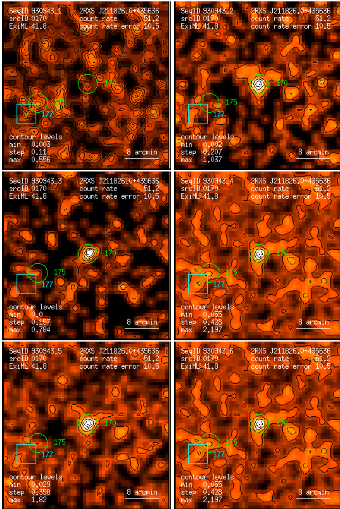
Figure 170: RASS 930943: detection 0170: band rate images, Gaussian filter: (1) PSPC channels 11 – 41, (2) 52 – 90, (3) 91 – 201, (4) 11 – 235, (5) 52 – 201, (6) 11 – 201. Broad band rates in counts/ks. Band rate contour levels in counts/ks/arcmin 2 .
