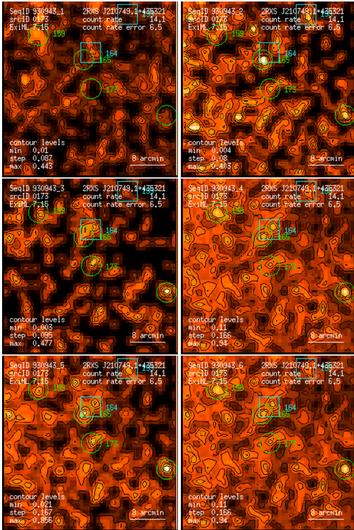
Figure 173: RASS 930943: detection 0173: band rate images, Gaussian filter: (1) PSPC channels 11 – 41, (2) 52 – 90, (3) 91 – 201, (4) 11 – 235, (5) 52 – 201, (6) 11 – 201. Broad band rates in counts/ks. Band rate contour levels in counts/ks/arcmin 2 .
