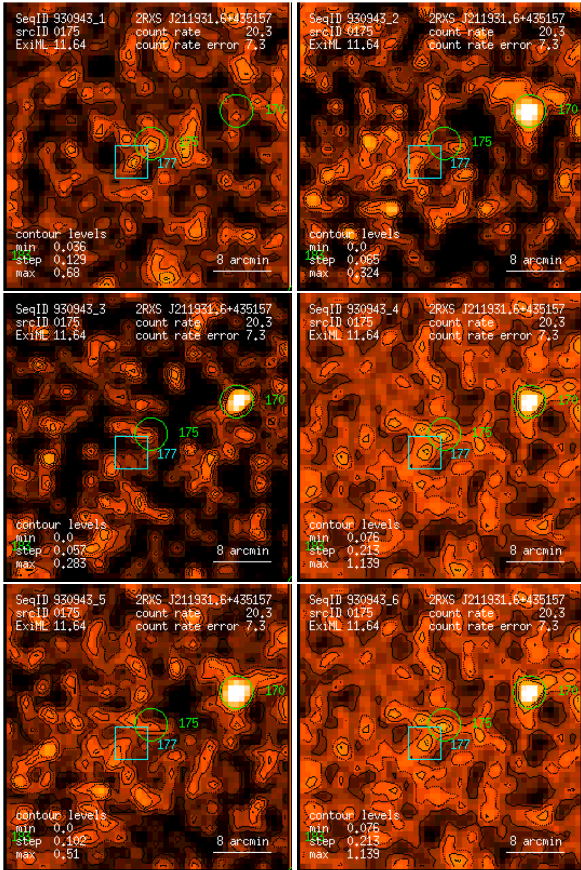
Figure 175: RASS 930943: detection 0175: band rate images, Gaussian filter: (1) PSPC channels 11 – 41, (2) 52 – 90, (3) 91 – 201, (4) 11 – 235, (5) 52 – 201, (6) 11 – 201. Broad band rates in counts/ks. Band rate contour levels in counts/ks/arcmin 2 .
