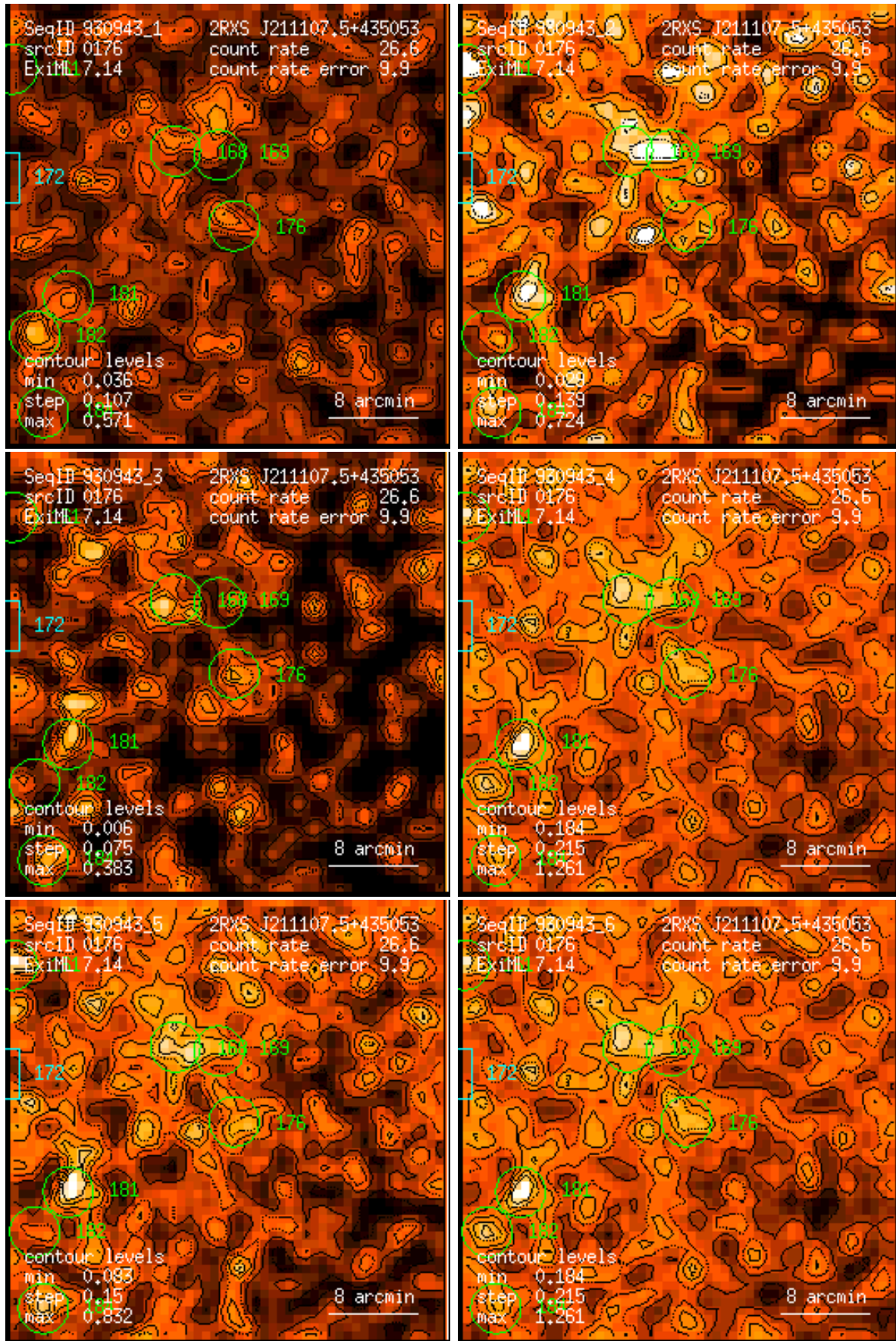
Figure 176: RASS 930943: detection 0176: band rate images, Gaussian filter: (1) PSPC channels 11 – 41, (2) 52 – 90, (3) 91 – 201, (4) 11 – 235, (5) 52 – 201, (6) 11 – 201. Broad band rates in counts/ks. Band rate contour levels in counts/ks/arcmin 2 .
