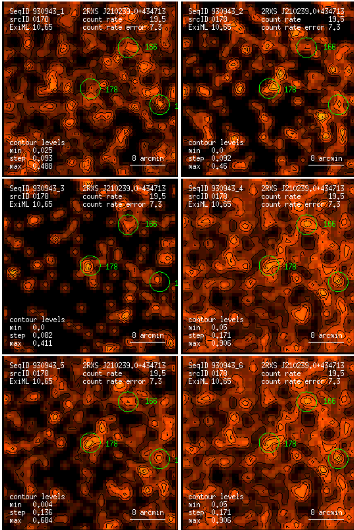
Figure 178: RASS 930943: detection 0178: band rate images, Gaussian filter: (1) PSPC channels 11 – 41, (2) 52 – 90, (3) 91 – 201, (4) 11 – 235, (5) 52 – 201, (6) 11 – 201. Broad band rates in counts/ks. Band rate contour levels in counts/ks/arcmin 2 .
