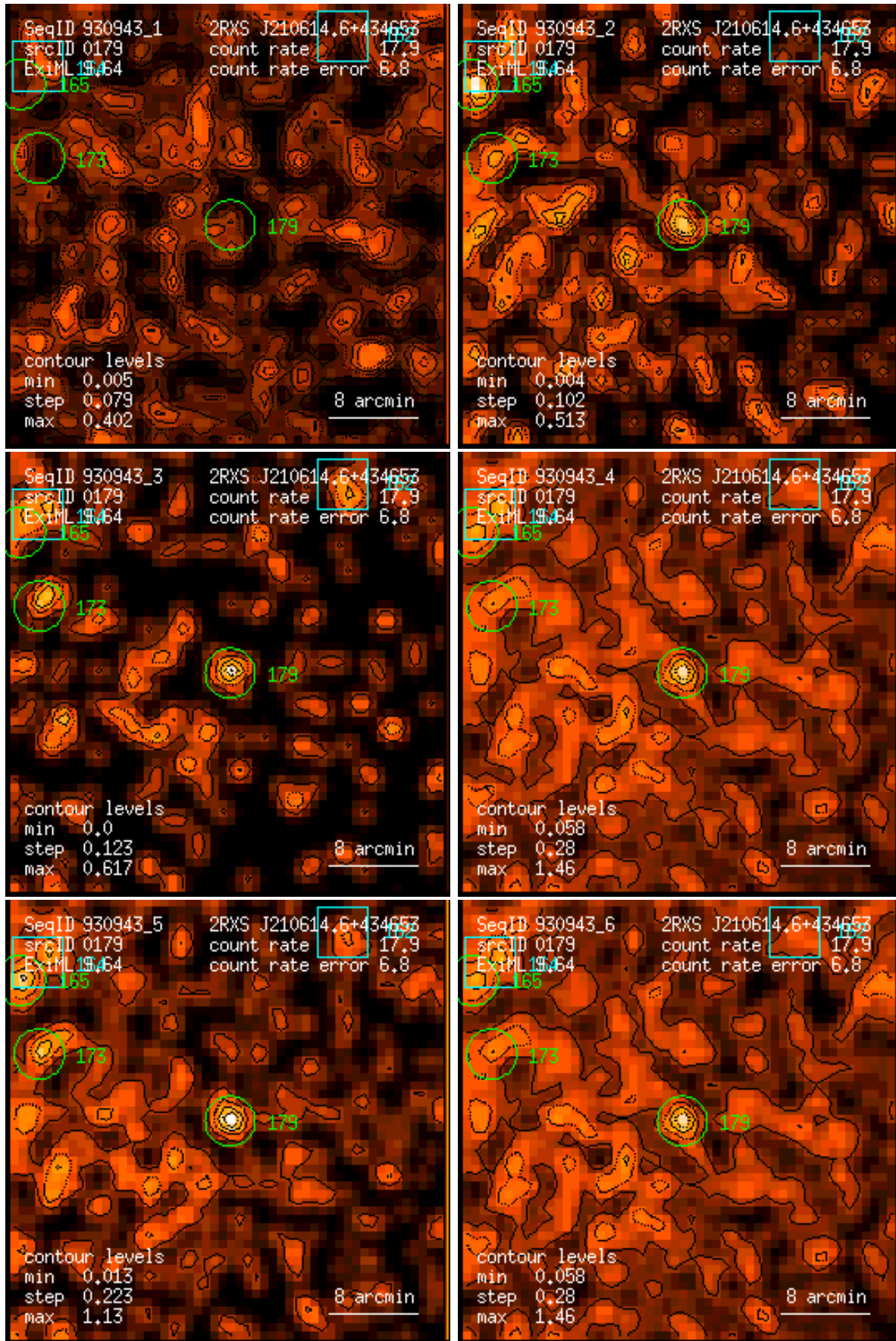
Figure 179: RASS 930943: detection 0179: band rate images, Gaussian filter: (1) PSPC channels 11 – 41, (2) 52 – 90, (3) 91 – 201, (4) 11 – 235, (5) 52 – 201, (6) 11 – 201. Broad band rates in counts/ks. Band rate contour levels in counts/ks/arcmin 2 .
