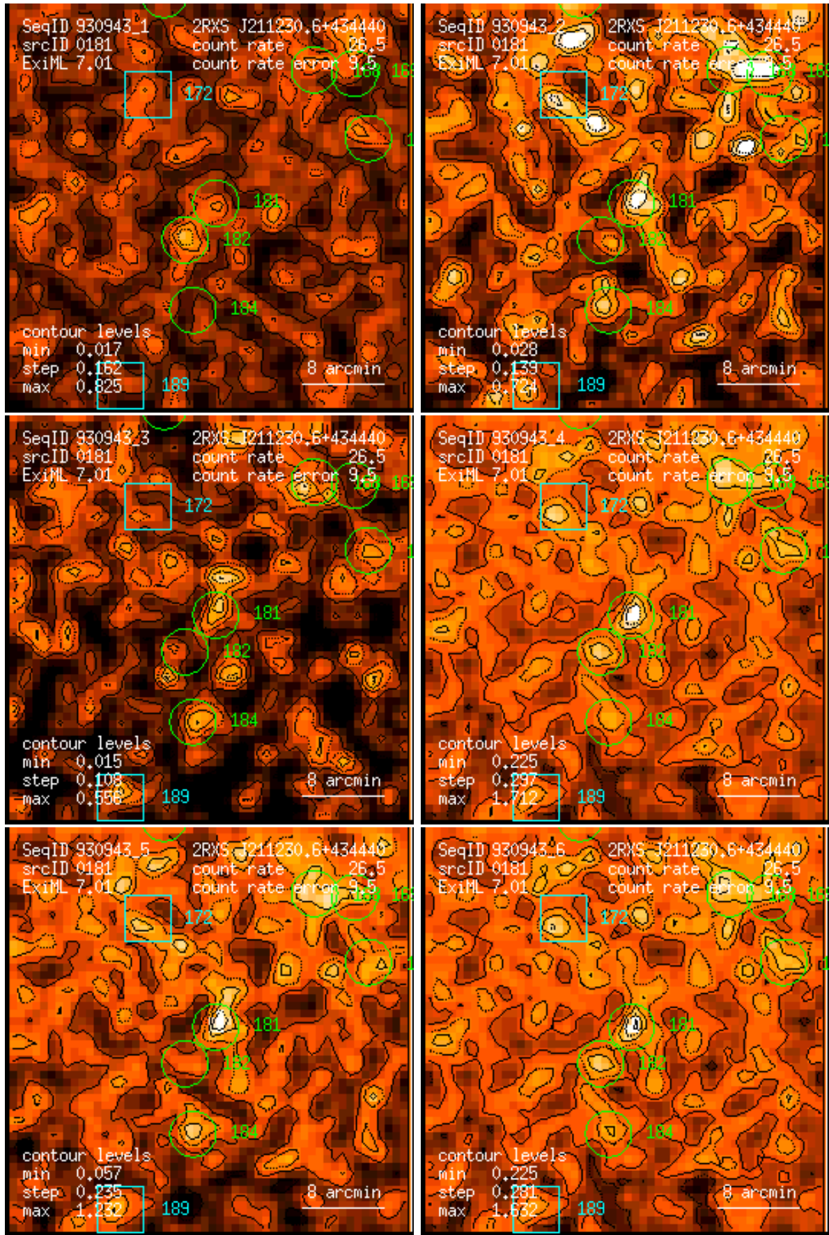
Figure 181: RASS 930943: detection 0181: band rate images, Gaussian filter: (1) PSPC channels 11 – 41, (2) 52 – 90, (3) 91 – 201, (4) 11 – 235, (5) 52 – 201, (6) 11 – 201. Broad band rates in counts/ks. Band rate contour levels in counts/ks/arcmin 2 .
